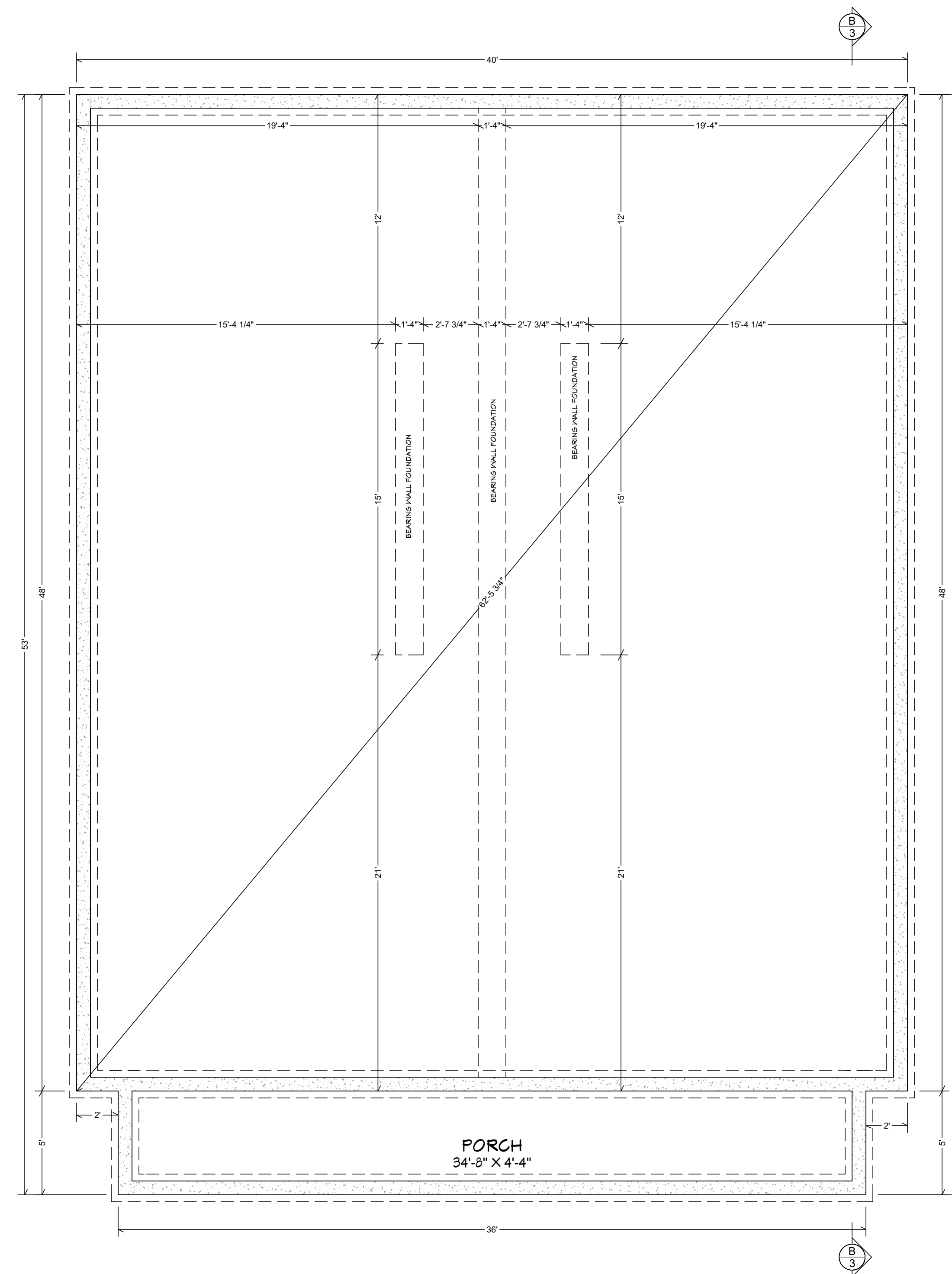
FOUNDATION PLAN
