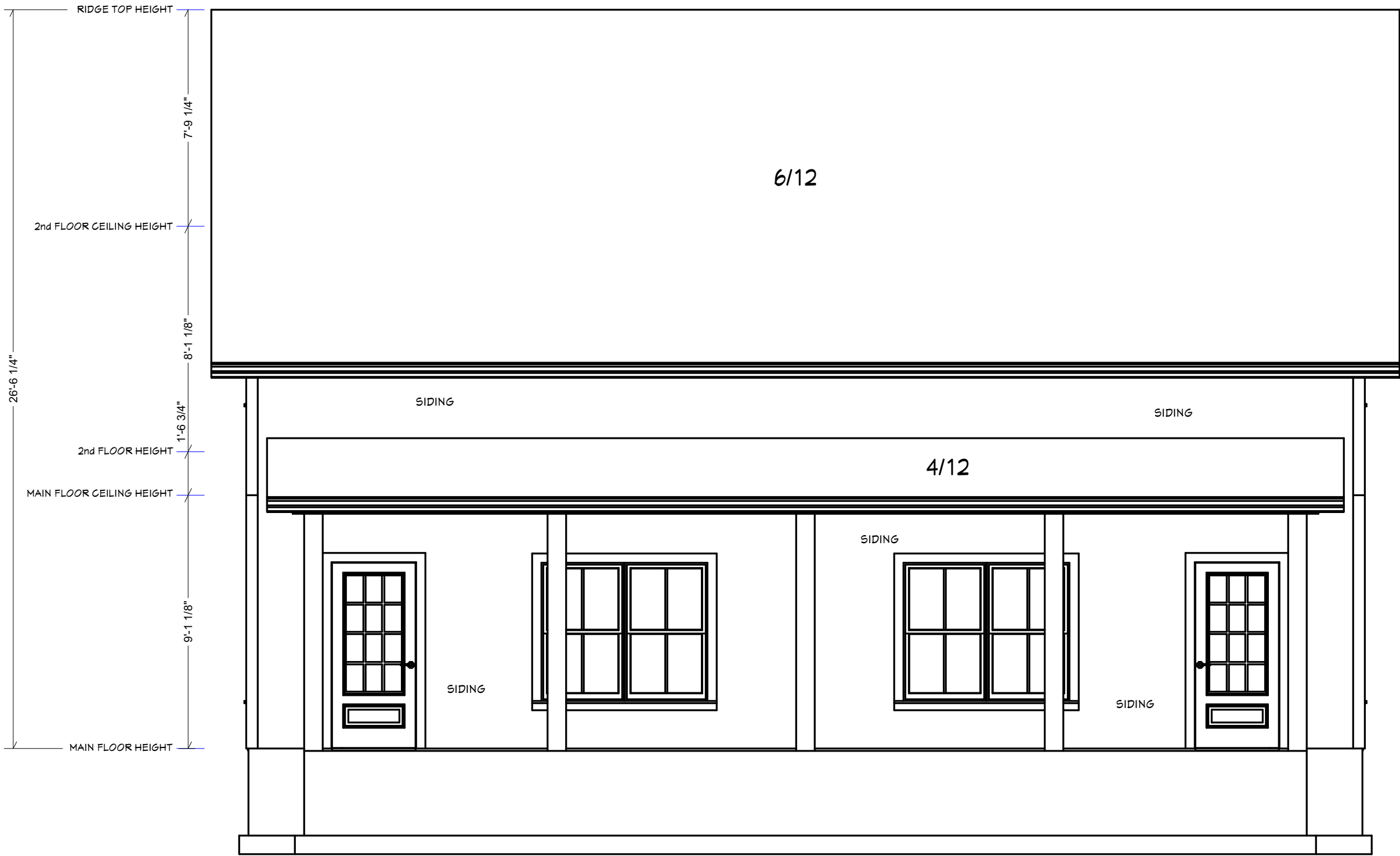
FRONT ELEVATION SCALE: 1/4" = 1'
