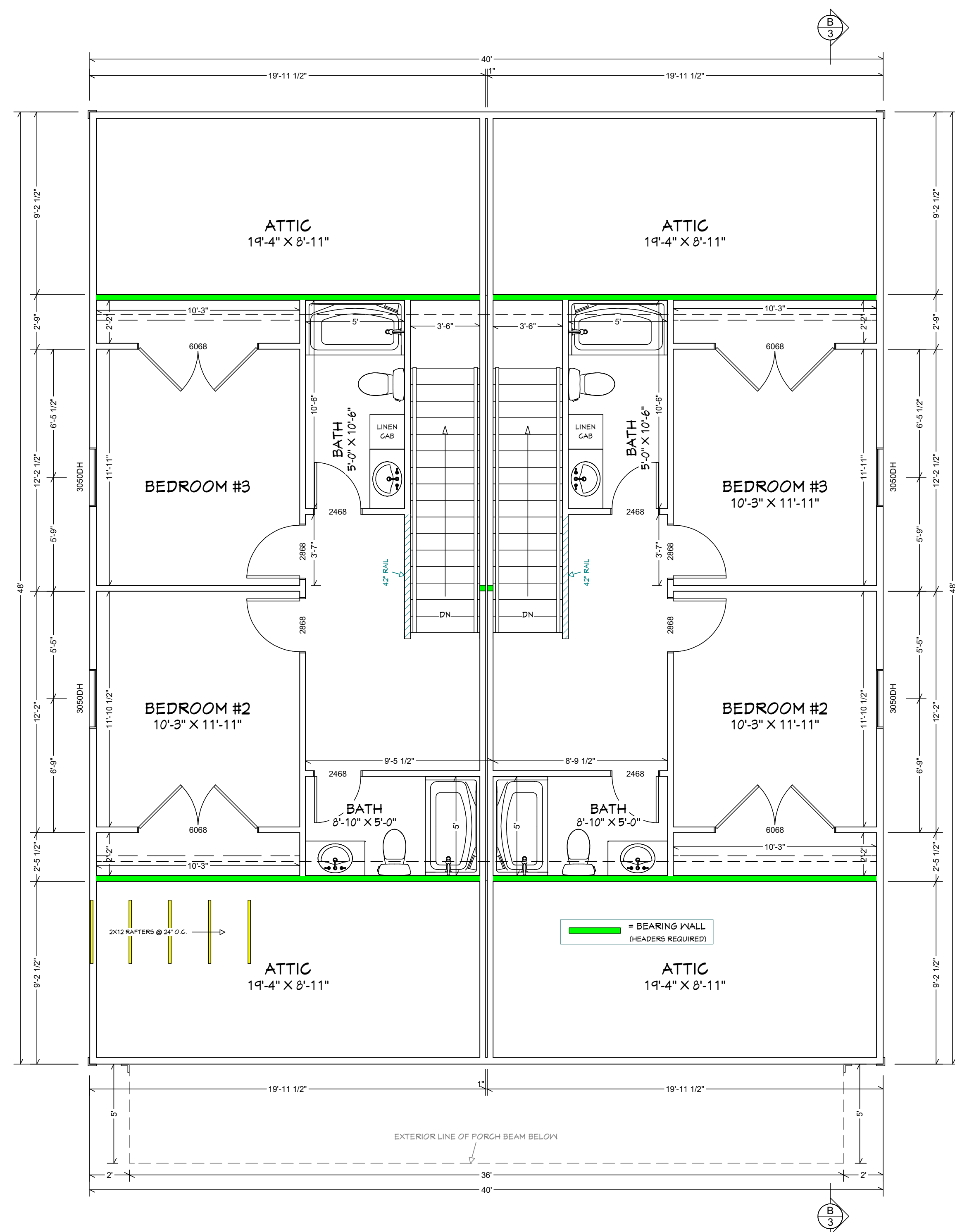
2ND FLOOR PLAN LIVING AREA 1076 SQ FT SCALE: 1/4" = 1'
