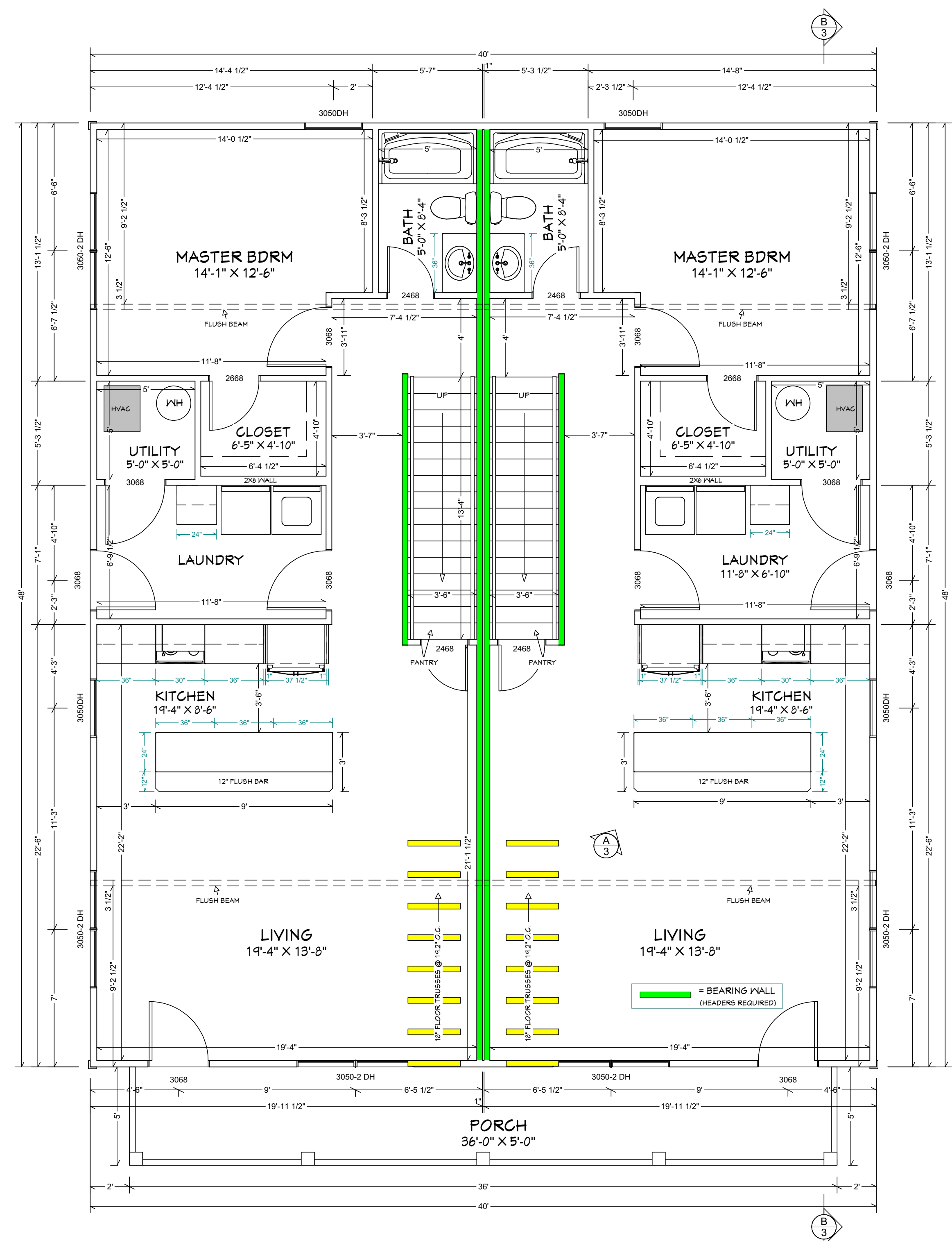
MAIN FLOOR PLAN LIVING AREA 1920 SQ FT SCALE: 1/4" = 1'
