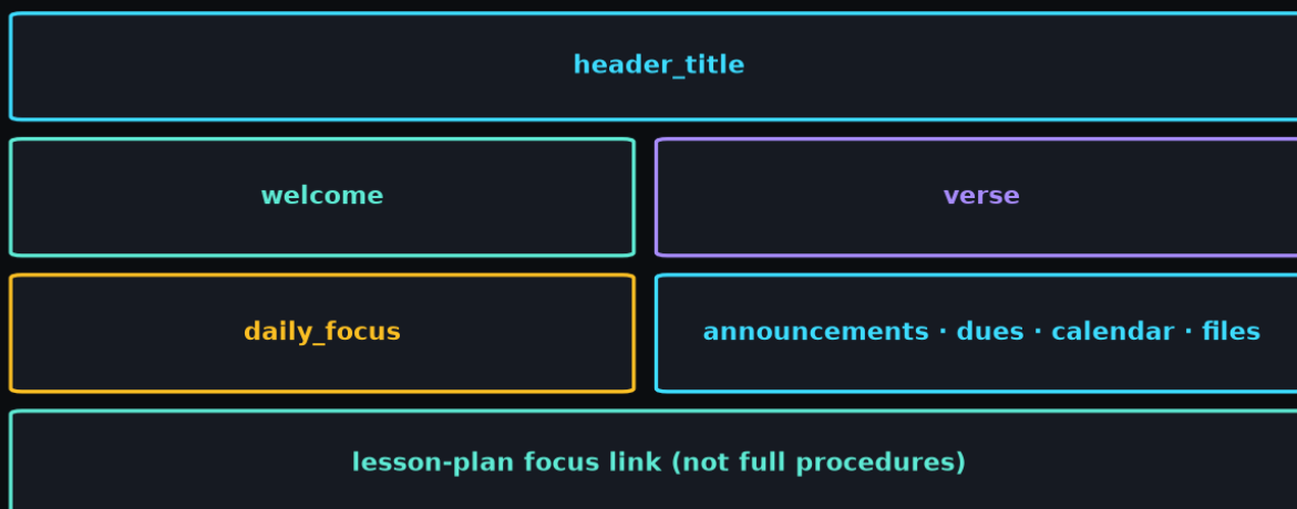
Figure: Named regions + live join layout.
