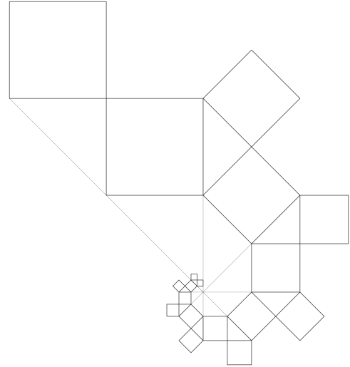
Figure 2: Negative orbit with hypotenuse line construction.
