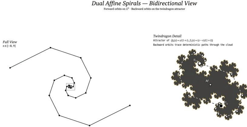
Figure 6: Bidirectional view: forward orbits ( n \geq 0 ) expand outward on the integer lattice \mathbb{Z}^2 , while backward orbits ( n < 0 ) trace deterministic paths that densely fill the Twindragon attractor.
