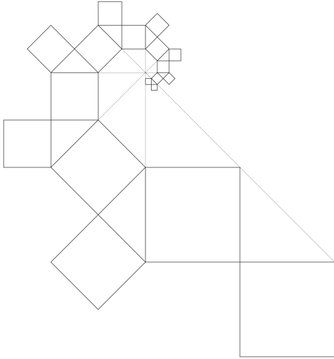
Figure 1: Positive orbit with hypotenuse line construction.
