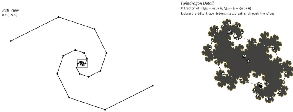
Figure 6: Bidirectional view: forward orbits ( n \geq 0 ) expand outward on the integer lattice \mathbb{Z}^2 , while backward orbits ( n < 0 ) trace deterministic paths that densely fill the Twindragon attractor.
