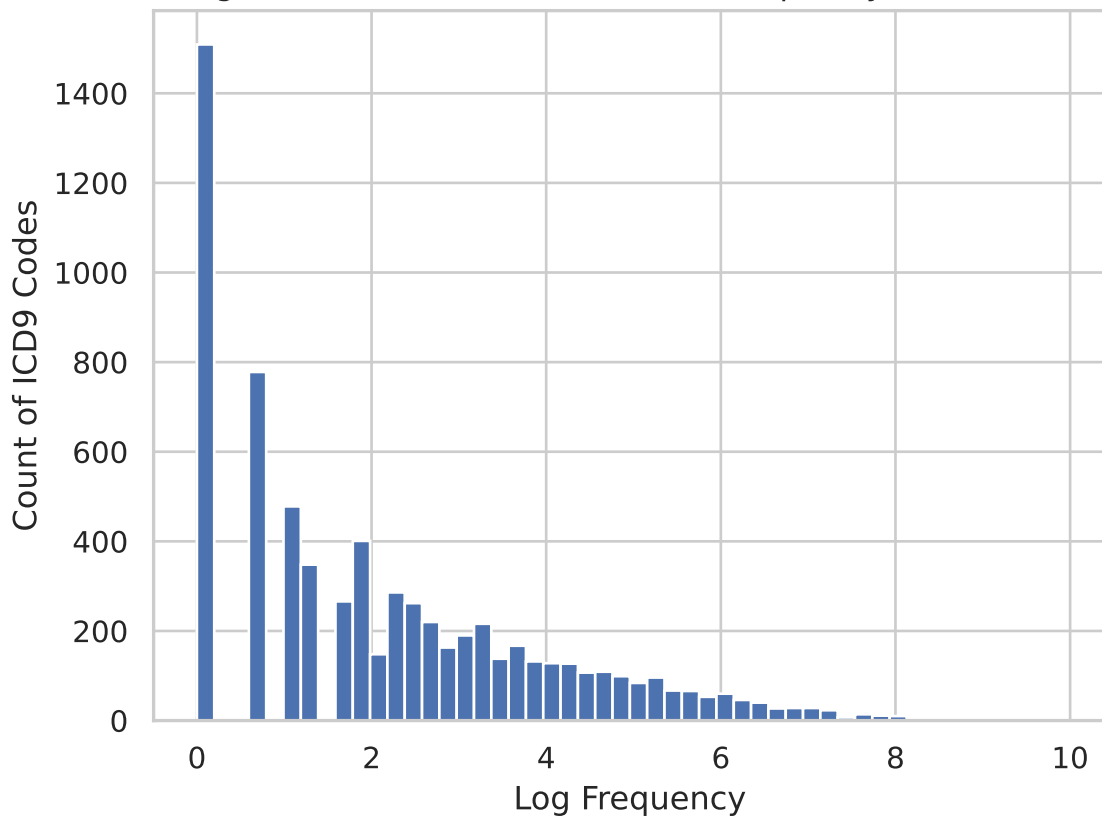
Log-Transformed Train ICD9 Code Frequency Distribution
