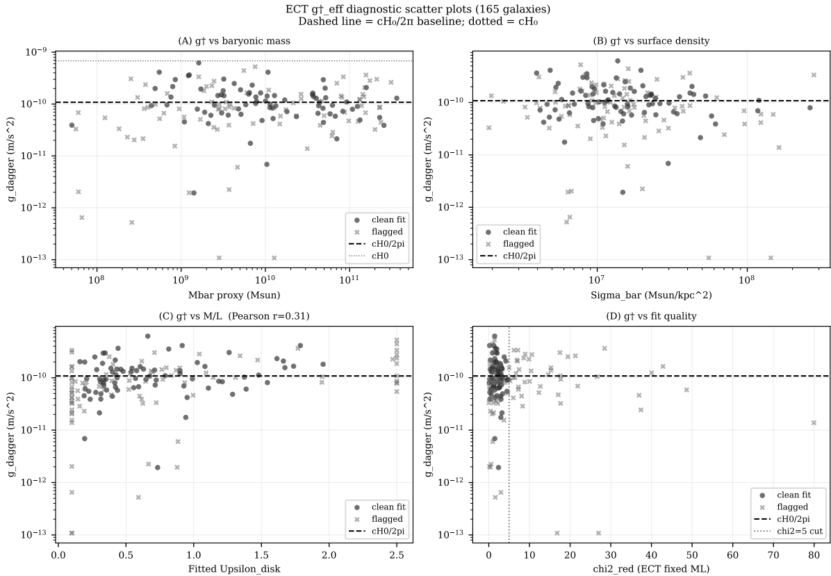
Figure 52: Additional scatter diagnostics for the fitted effective critical scale g_{\text{eff}}^{\dagger} across the SPARC sample: dependence on a baryonic mass proxy, a baryonic surface-density proxy, the fitted disk mass-to-light ratio, and the fit quality itself. These plots are retained as supplementary diagnostics rather than promoted to the main text, because the more compact summary is now given by Fig. 25.
