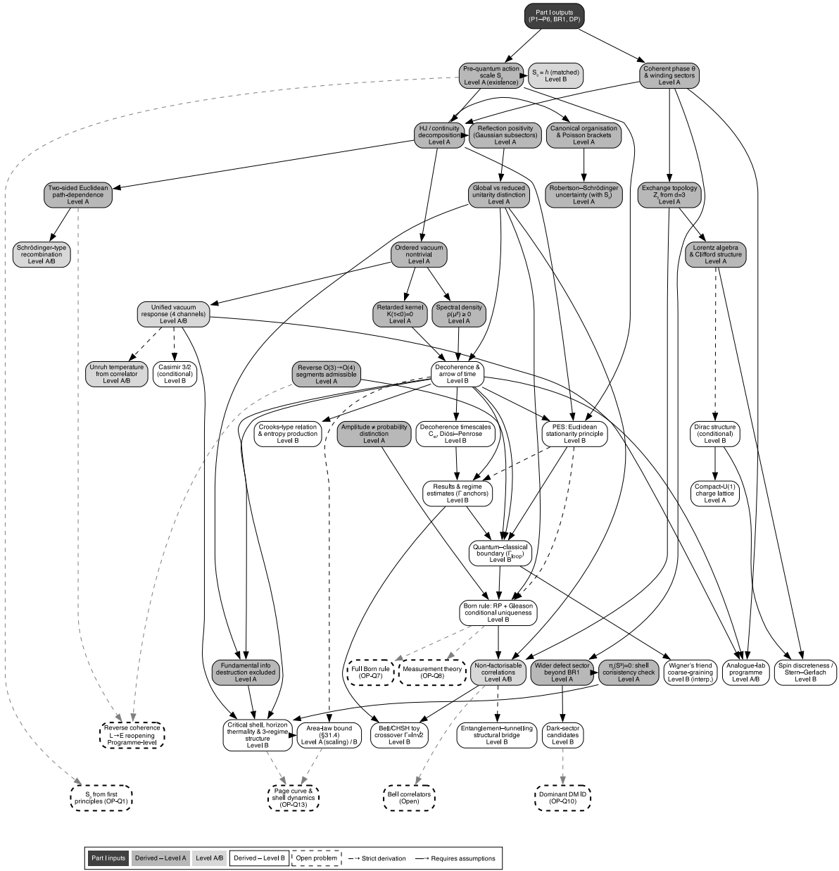
Figure 19: Part III derivation logic, updated with the QG/decoherence upgrade layer. The coherent branch develops structural routes to Hilbert-space structure, wave equations, Born-type weighting, decoherence, PES, vacuum effects, black-hole thermodynamics, and measurement-status analysis. Born weights remain conditional on the RP/Gleason/decoherence route, and a complete measurement-update theorem remains open. The reduced-state upgrade layer comprises the hybrid-consistency architecture and two-level ontology (§38), the gravity-induced-entanglement operational criterion (§39), the \phi vs \delta n_A mediator taxonomy (§40), the BMS/memory/soft-graviton infrared sector (§41), the islands/QES structural mapping with the critical shell (discussed within the BH section), and the open orientation-sector entangling-mediator task (OP-Q22). Colours indicate derivation levels.
