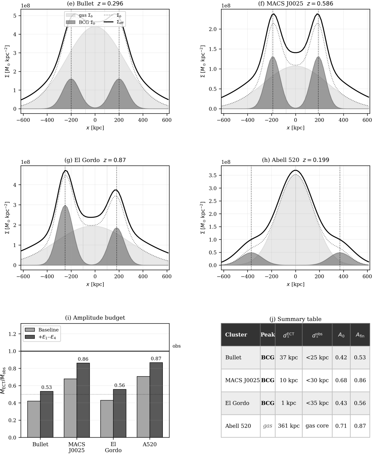
Figure 14: Four-system order/argmax-preservation audit with toy Gaussian baryonic inputs. The plotted A_0^{\text{proxy}} and A_{\text{fin}}^{\text{proxy}} are deterministic hand-set normalisation sensitivities, not observational amplitudes.
