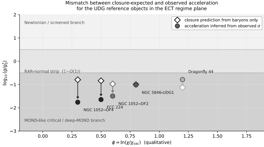
Figure 11: Direct acceleration-residual view for the UDG reference objects. The comparison uses g_{\text{obs}} = 3\sigma^2/R_{1/2} and the adopted Level-C closure; it assigns no microscopic scalar coordinate and is not a screening result.
