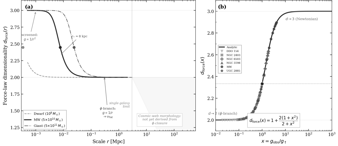
Figure 17: Force-law effective dimensionality in ECT. (a) d_{\text{force}}(r) for three galaxy masses, computed analytically from the \phi -closure \mu(g_{\text{obs}}/g_\dagger)g_{\text{obs}} = G_N M/r^2 . In the screened regime ( g_{\text{obs}} \gg g_\dagger ): d_{\text{force}} \rightarrow 3 (Newtonian). Beyond the transition radius r_* = \sqrt{G_N M/g_\dagger} (filled dots): d_{\text{force}} \rightarrow 2 ( g \propto 1/r \Rightarrow v_{\text{flat}} = \text{const} ). At r_* (where x = g_{\text{obs}}/g_\dagger = 1 ): d_{\text{force}} = 7/3 \approx 2.33 . Curves fade beyond the isolation radius ( \sim 1\text{--}3 Mpc), where the single-galaxy approximation breaks down. The shaded region at r > 3 Mpc indicates cosmic-web scales where d_{\text{force}} is not yet derivable from the present \phi -closure. (b) Universal curve d_{\text{force}}(x) with the closed-form analytic expression d_{\text{force}} = 1 + 2(1+x^2)/(2+x^2) ; every galaxy falls on the same curve, because the formula depends only on x = g_{\text{obs}}/g_\dagger , not on M or r separately. Different galaxies differ only in the mapping x(r) : heavier galaxies reach higher x at any given r . This universality is the dimensionality counterpart of the radial acceleration relation.
