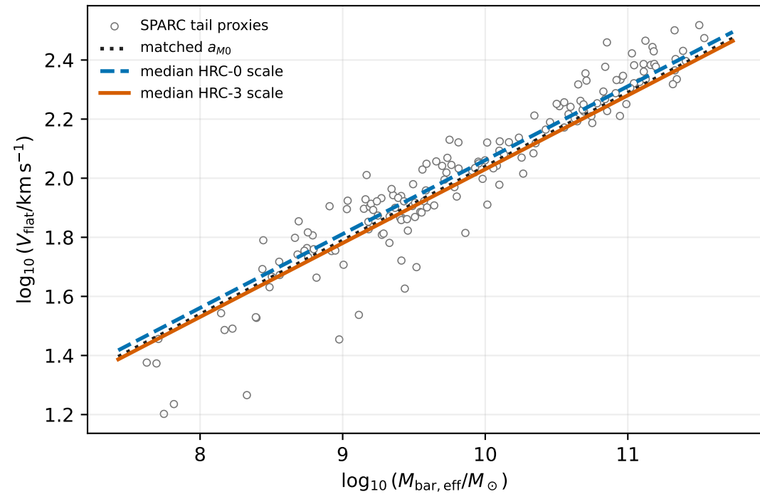
Conditional BTFR and tail proxies
