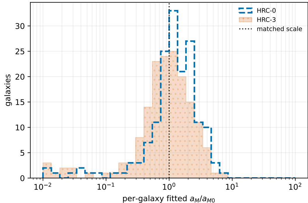
Algebraic scale dispersion
