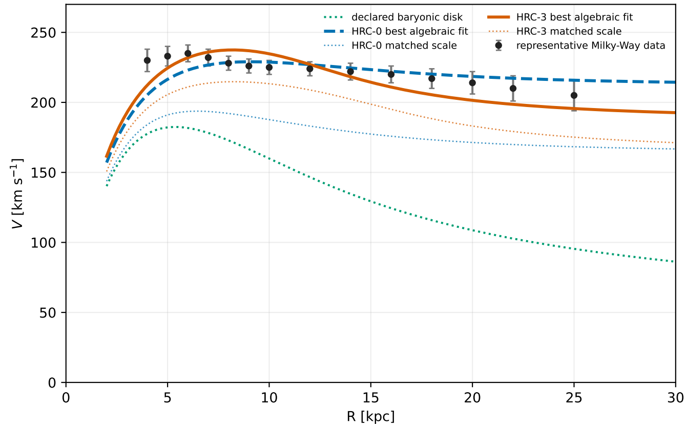
Milky Way: HRC-only algebraic sensitivity test
