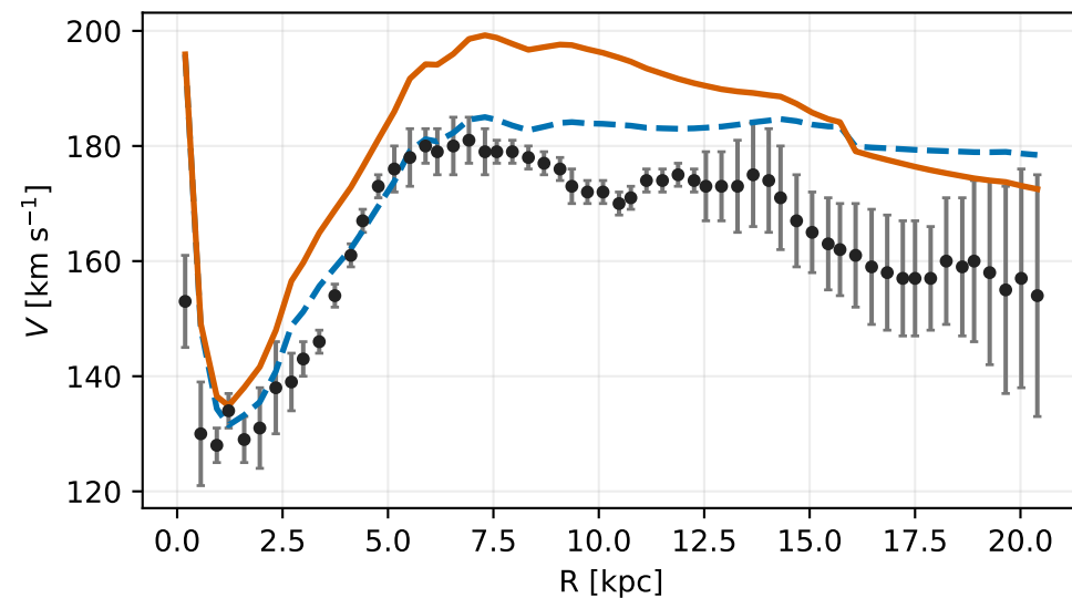
NGC6946
