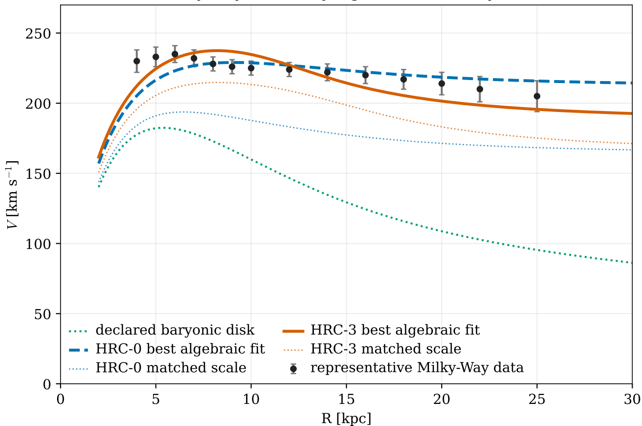
Milky Way: HRC-only algebraic sensitivity test
