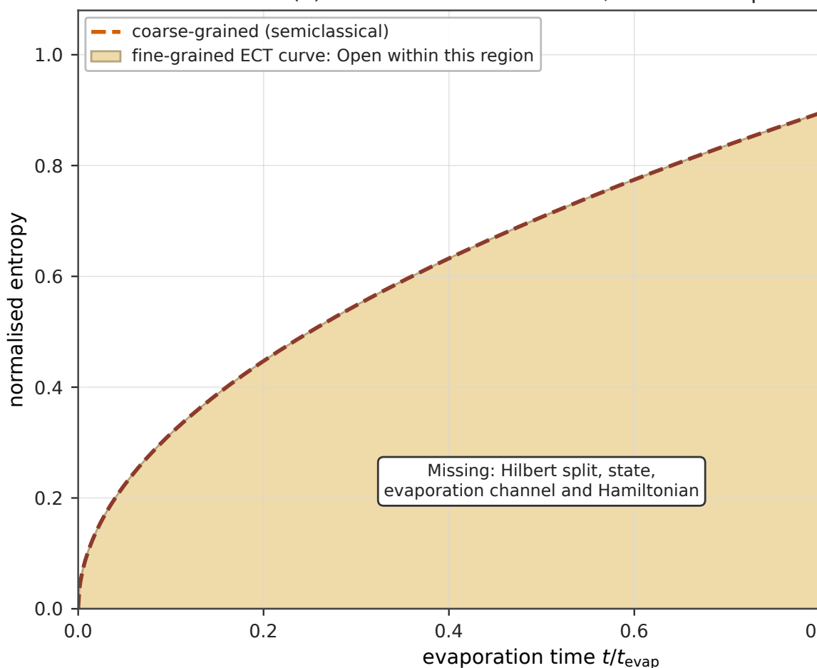
(b) Semiclassical benchmark; ECT curve Open
