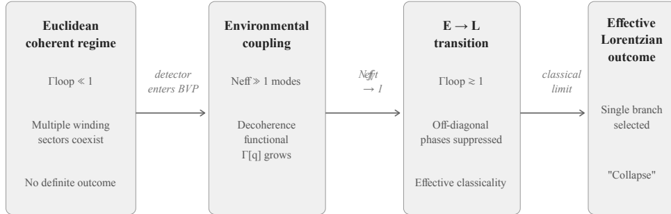
Figure 43: Structural reading of quantum measurement in ECT as a Euclidean-to-Lorentzian transition. In the coherent regime ( \Gamma_{\text{loop}} \ll 1 ) multiple winding sectors coexist without a definite outcome. Environmental coupling to N_{\text{eff}} \gg 1 modes drives the decoherence functional \Gamma[q] to grow. When \Gamma_{\text{loop}} \gtrsim 1 the off-diagonal interference terms are suppressed and an effectively classical (Lorentzian) single-branch outcome is selected. This should be read as a structural flow, not as a completed microscopic derivation of realistic detector dynamics.
