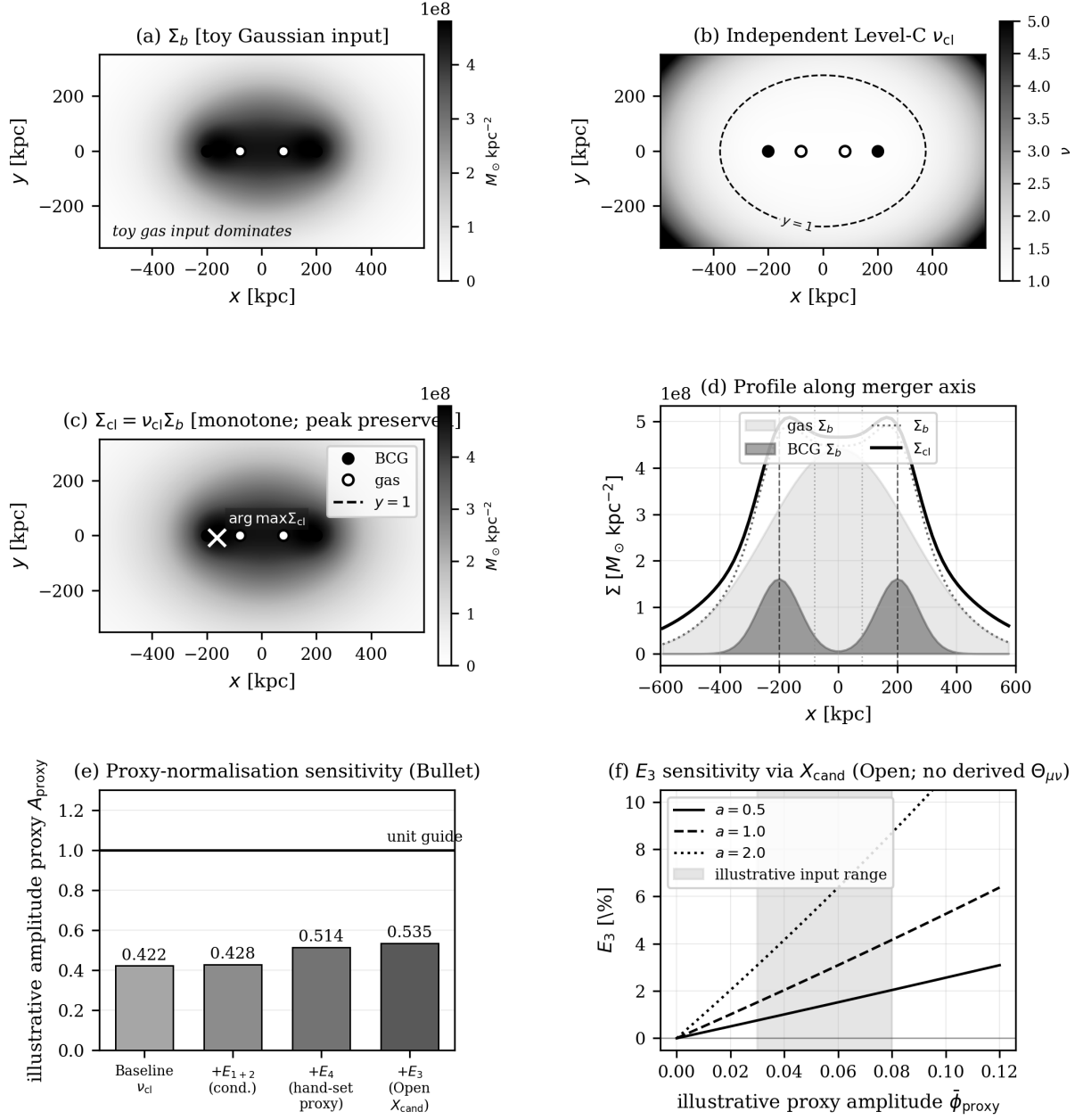
Markers = centres of hand-set toy BCG/gas Gaussians; masses, widths, and offsets are not reconstructed baryon likelihoods Bullet inputs: g_{cl}^1 = 1.2 \times 10^{-10} \text{ m s}^{-2} , hand-set A_{obs}^{proxy} = 3.0 ; amplitudes are illustrative proxies \Sigma_{cl}(\Sigma_b) is monotone: peak preservation is a tautological sanity check, not morphology evidence
