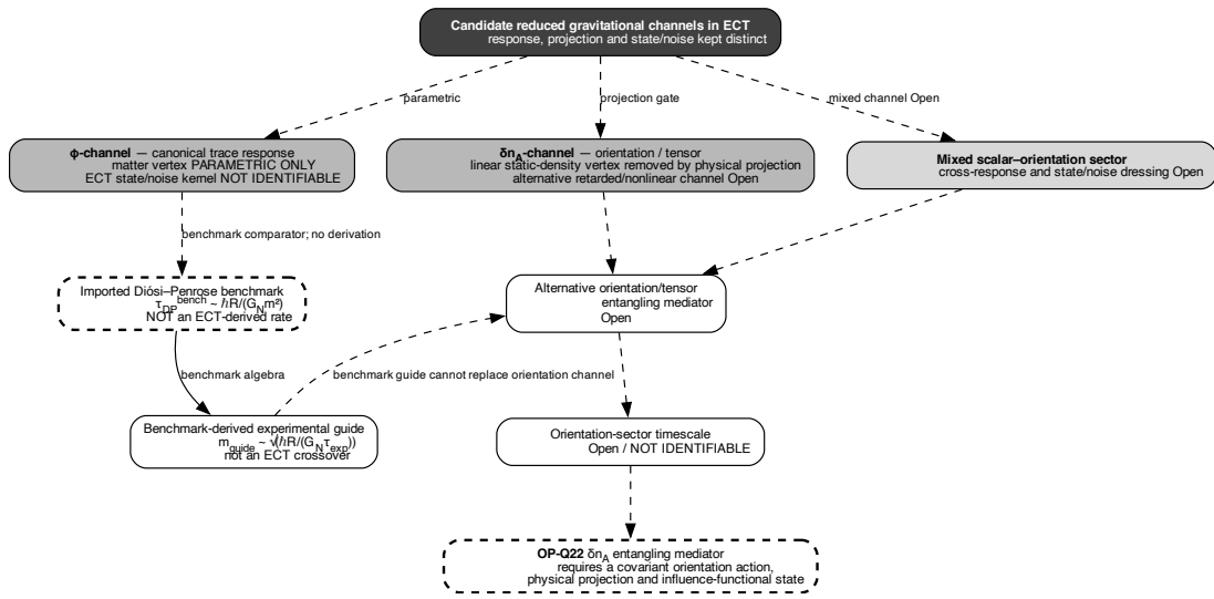
Figure 37: Status taxonomy of candidate reduced gravitational channels. The scalar branch contains a parametric trace response but no identified ECT noise/state; the Diósi–Penrose rate and m_{\text{guide}} are external benchmarks. The projected linear static-density orientation route has a missing vertex, while alternative retarded/nonlinear orientation and mixed channels remain Open. Solid and dashed arrows denote established algebra inside the stated model and missing matching/state steps, respectively.
