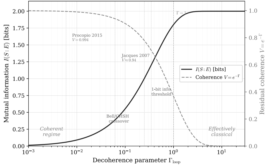
Figure 36: Qubit information–decoherence trade-off in the ECT dephasing closure (Eq. 30.4). Solid curve: mutual information I(S:E) in bits as a function of the decoherence parameter \Gamma_{\text{loop}} . Dashed curve: residual coherence V = e^{-\Gamma} (right axis). Vertical dotted lines mark operational anchors from ECT-calibrated experiments: Procopio 2015 ( V = 0.994 , quantum switch), Jacques 2007 ( V \approx 0.94 , delayed-choice interferometer), the one-bit information threshold ( \Gamma \approx 0.25 ), and the Bell/CHSH crossover ( \Gamma = \ln \sqrt{2} \approx 0.35 ). The dashed vertical line at \Gamma = 1 separates the coherent and effectively classical regimes. This is a Level B closure result for the specific dephasing model, not a protocol-independent theorem. Numerical details are given in Appendix BB.
