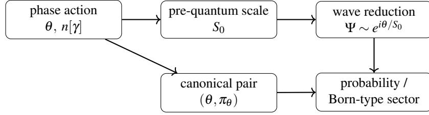
Figure 30: Structural roadmap of the coherent-sector quantization logic in ECT (Level B). Phase dynamics and loop quantization prepare the action scale S_0 , which supports wave reduction, canonical structure, and eventually the Born-type reduced probability sector. The figure is a structural roadmap rather than a closed derivation of S_0 = \hbar .
