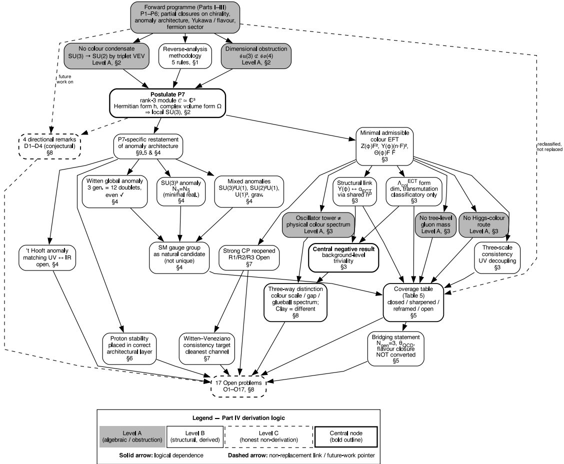
Figure 43: Derivation logic of Part IV (Reverse Analysis, SU(3) Completion, and Structural Constraints). The diagram is organised into four layers: (i) the forward inputs from Parts I–III (the postulates P1–P6 and the partial closures they support); (ii) the reverse-analysis layer (the obstruction theorems forcing externalisation of colour, and the formalisation of P7); (iii) the structural-consequences layer (the minimal admissible colour EFT, its obstruction theorems, the dimensional-transmutation form of \Lambda_{col}^{ECT} , the central background-level triviality result, and the anomaly-consistency layer); and (iv) the status layer (coverage reclassification, proton stability placed in the correct layer, strong CP reopened, and the tabular closures/open/directional ledgers). Node shading: dark = Level A (algebraic or obstruction), light = Level B (structural/derived within reverse analysis), dashed outline = Level C or honest non-derivation. Solid arrows denote logical dependence; dashed arrows denote the non-replacement connection to the forward programme of Parts I–III.
