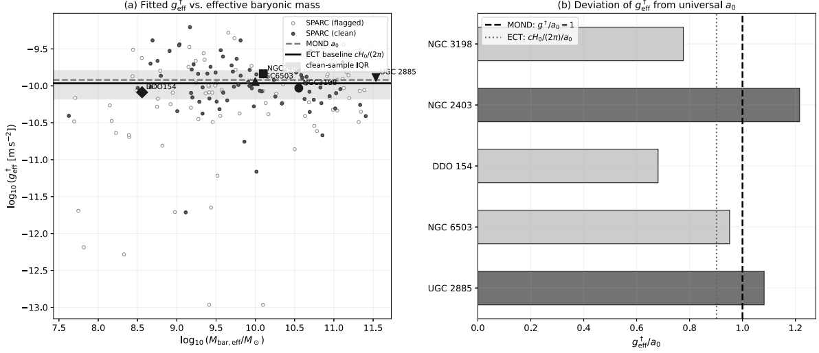
Figure 24: Summary of the fitted effective critical scale in the galactic pipeline. Panel (a) compares the fitted g_{\text{eff}}^{\dagger} values with the matched reference g_0^{\dagger} = cH_0/(2\pi) and the MOND reference a_0 ; panel (b) shows representative fit ratios. The scatter is a data-interface output, not a derived environment signal or evidence that non-universality is physical.
