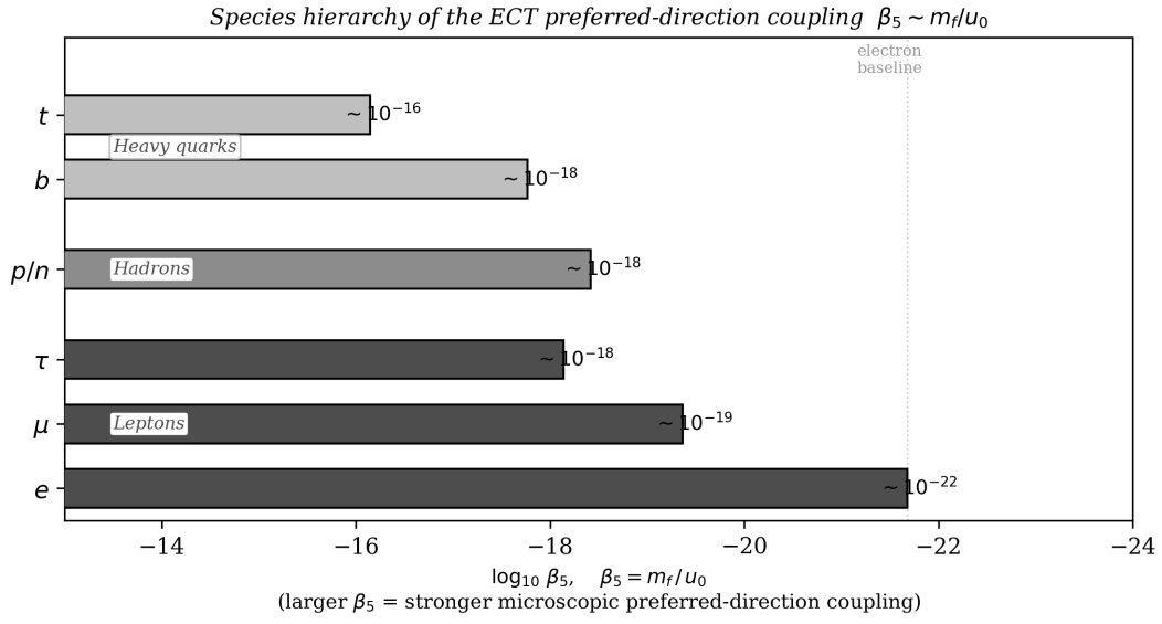
Figure 4: Species dependence of the ECT preferred-direction coupling in the present EFT scaling \beta_5 \sim m_f/\phi_0 . Heavier fermionic species correspond to larger dimensionless ratios \beta_5 , although all values remain extremely small because the suppression scale is the radial symmetry-breaking scale \phi_0 \sim \bar{M}_{\text{Pl}} . The figure is schematic and illustrates parametric hierarchy rather than a precision prediction for observable signals.
