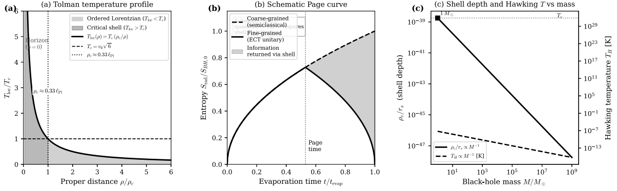
Figure 39: ECT black-hole information scenario. (a) Tolman temperature profile T_{\text{loc}}(\rho) near a non-extremal horizon, plotted in units of T_c vs. \rho/\rho_c . The condensate critical temperature T_c = \phi_0 \sqrt{6} (dashed horizontal line) is reached at the universal proper distance \rho_c \approx 0.33 \ell_{\text{Pl}} (dotted vertical line), independently of the black-hole mass. The lightly shaded region is the well-ordered Lorentzian phase ( T_{\text{loc}} < T_c ); the darker shaded region marks the near-horizon critical shell ( T_{\text{loc}} > T_c ). (b) Schematic Page curve. The coarse-grained radiation entropy (dashed) rises monotonically as in the semiclassical Hawking approximation. The fine-grained entropy (solid) follows the coarse-grained branch until the Page time, then decreases as the shell entropy capacity becomes finite and state-dependent corrections to emission become order-one. The shaded area between the two curves represents entropy that is “returned” via shell-mediated correlations. The figure is schematic; a quantitative curve requires the explicit shell Hamiltonian. (c) Black-hole parameters vs. mass. The critical shell proper distance \rho_c is mass-independent (not shown separately); the ratio \rho_c/r_s \propto M^{-1} (left axis, red) shows how deeply the shell is buried inside the Schwarzschild radius. The Hawking temperature T_H \propto M^{-1} (right axis, dashed blue) decreases with mass. For all astrophysical black holes T_H \ll T_c ; the critical shell is firmly in the sub-Planckian regime.
