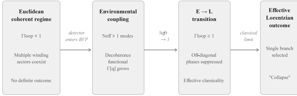
Figure 42: Structural reading of quantum measurement in ECT as a Euclidean-to-Lorentzian transition. In the coherent regime ( \Gamma_{\text{loop}} \ll 1 ) multiple winding sectors coexist without a definite outcome. Environmental coupling to N_{\text{eff}} \gg 1 modes drives the decoherence functional \Gamma[q] to grow. When \Gamma_{\text{loop}} \gtrsim 1 the off-diagonal interference terms are suppressed and an effectively classical (Lorentzian) single-branch outcome is selected. This should be read as a structural flow, not as a completed microscopic derivation of realistic detector dynamics.
