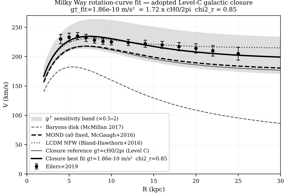
Figure 25: Milky Way rotation-curve fit in the adopted Level-C galactic closure. The figure compares the best-fit ECT curve, the baseline g^\dagger_0 = cH_0/(2\pi) curve, the baryonic disk model, and the MOND and \Lambda CDM comparison curves from the same numerical pipeline. The shaded/supplementary sensitivity band, where shown, represents only order-unity variations of the effective critical scale and is not interpreted here as a completed physical EFE calculation. The best-fit effective critical scale is g^\dagger_{\text{eff}} \approx 1.72 g^\dagger_0 .
