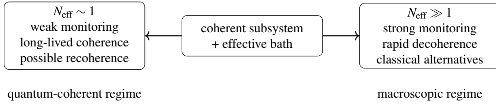
Figure 32: Qualitative regime split in the decoherence sector of ECT (Level B). When only a few effective environment channels are active ( N_{\text{eff}} \sim 1 ), coherence can survive for long times and recoherence is not excluded. When many channels effectively monitor the subsystem ( N_{\text{eff}} \gg 1 ), the reduced dynamics becomes strongly irreversible and classical-looking. This figure is schematic and summarises the logic developed in Section 26.1.
