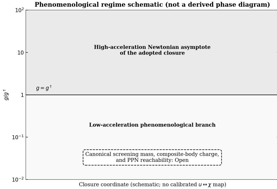
Figure 18: Status diagram for the galactic programme. The vertical axis shows only the two imposed acceleration regimes of the adopted Level-C fit. The horizontal scalar-closure axis has no calibrated physical coordinate: neither u \leftrightarrow \chi nor S \rightarrow G has been derived. The Open gate collects the required finite-body solution, scalar charge, screening trend, PPN test, and galactic source/force normalisation.
