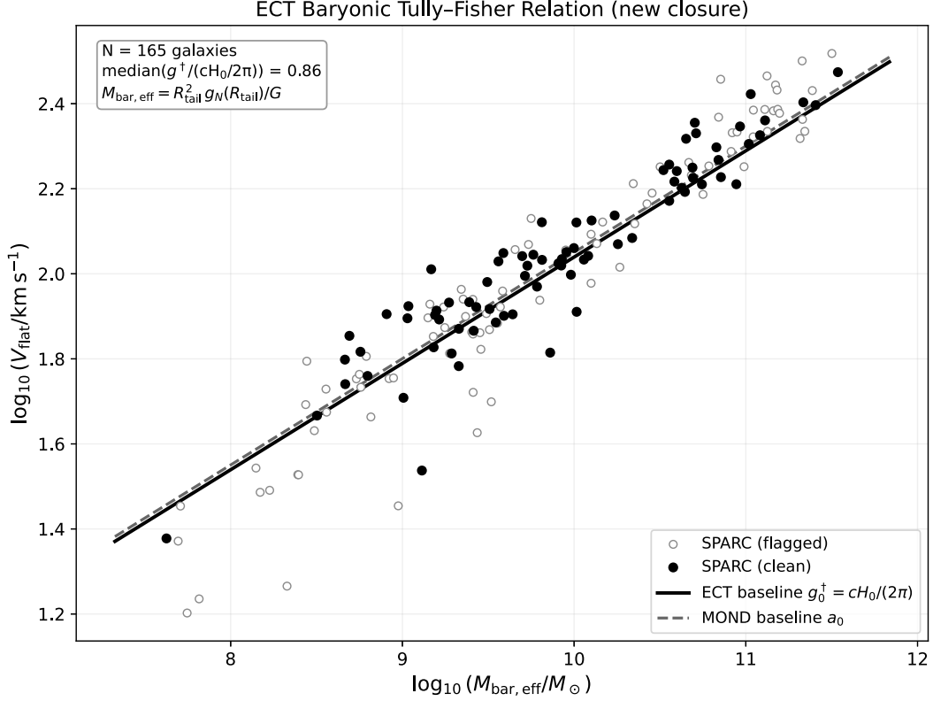
Figure 21: Internal BTFR diagnostic of the adopted Level-C SPARC closure. The points show the effective outer baryonic-mass proxy M_{\text{bar,eff}} = R_{\text{tail}}^2 g_N(R_{\text{tail}})/G_N inferred from the same baryonic decomposition used in the rotation-curve fits, plotted against V_{\text{flat}} . The solid line is the closure relation V_{\text{flat}}^4 = G_N M_{\text{bar,eff}} g_0^\dagger with the matched benchmark g_0^\dagger = cH_0/(2\pi) ; the dashed line uses the MOND reference a_0 . This self-consistency plot is not an independent catalogue-level BTFR test and does not establish an ECT derivation of the functional or normalisation.
