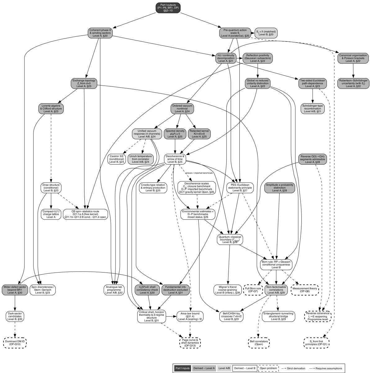
Figure 40: Derivation logic of Part III (Quantum Sector). Starting from Part I inputs inherited through BR1, the diagram organises the quantum sector into its main structural blocks: coherent phase dynamics and S_0 ; Hamilton-Jacobi / continuity; reflection positivity and the Hilbert-space bridge; canonical organisation and uncertainty; exchange topology and Dirac closure; ordered-vacuum response (Casimir, Unruh, particle production, horizon thermality); decoherence and the arrow of time; PES; the quantum-classical boundary; Born-type probability via Gleason; entanglement and Bell-type correlations; black-hole thermodynamics and information exclusion; the analogue-laboratory programme; and the QG/decoherence upgrade layer (problem of time, ECT-specific falsifiers, reduced-state hybrid-consistency architecture, two-level ontology, gravity-induced entanglement with its operational criterion, mediator taxonomy with the \phi -channel and \delta n_A -channel distinction, IR/soft sector, islands/QES structural mapping onto the critical shell, and the cross-programme diagnostic discriminants). Node shading follows the same convention as Figure 29: dark = inherited Part I inputs, medium = Level A, light = Level A/B, white = Level B, dashed = open. Solid arrows = strict derivation; dashed arrows = closure-dependent steps.
