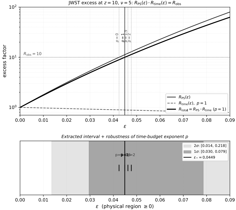
Figure 48: Decomposition of the JWST extraction into the two \varepsilon -dependent factors R_{\text{PS}}(\varepsilon) and R_{\text{time}}(\varepsilon) , under the common background module of Appendix AH. Upper panel: the Press-Schechter growth-enhancement factor R_{\text{PS}} rises monotonically with \varepsilon , while the stellar-assembly time-budget factor R_{\text{time}} decreases. Their product R_{\text{total}}(\varepsilon) (solid dark curve) crosses the observational target R_{\text{obs}} = 10 at \varepsilon \approx 0.045 . Lower panel: the extracted \varepsilon -interval [0.030, 0.079] ( 1\sigma , bracket on peak height \nu ) and [0.014, 0.218] ( 2\sigma , bracket on both \nu and R_{\text{obs}} ) shown as grayscale shaded bands. Robustness check of AG.4 also superposed as vertical lines at \varepsilon(p=0) , \varepsilon(p=1.5) , \varepsilon(p=2) . All shading and line styles are grayscale per preprint convention.
