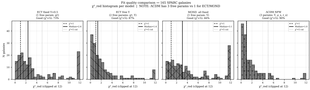
Figure 23: Fit-quality comparison across 165 SPARC galaxies for the new ECT galactic closure (fixed and free M/L modes), MOND, and \Lambda CDM/NFW. The fixed- M/L ECT mode provides the cleaner test of the galactic critical scale because it removes the strongest stellar disk M/L degeneracy, while the free- M/L mode shows the best-fit performance once that nuisance freedom is restored.
