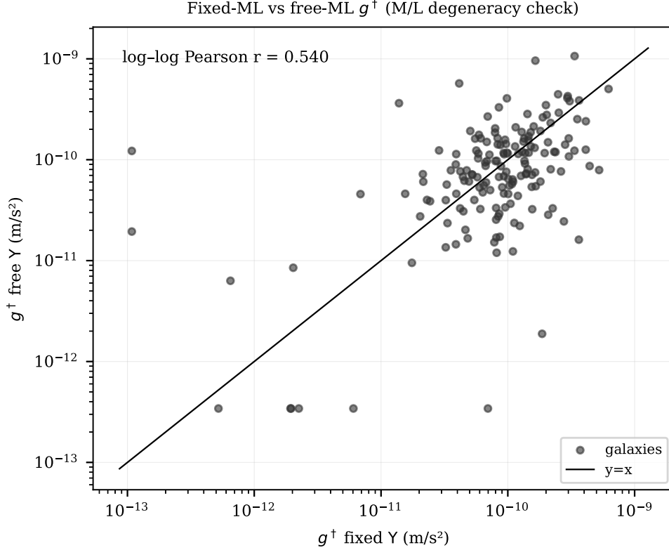
Figure 55: Fixed- M/L versus free- M/L comparison of the fitted effective critical scale g_{\text{eff}}^{\dagger} . The diagonal y = x marks identical recovered values. The moderate correlation indicates that part of the scatter in g_{\text{eff}}^{\dagger} is robust under changes in the disk mass-to-light treatment, while another part is clearly entangled with the M/L degeneracy. This is why the fixed- M/L mode is used in the main text as the cleaner test of the ECT galactic closure, whereas the free- M/L mode is interpreted as a robustness check rather than as the primary physical result.
