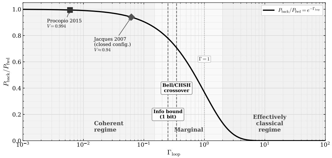
Figure 33: Operational crossover map organised by the decoherence parameter \Gamma_{\text{loop}} . The solid curve shows the reverse-coherence ratio P_{\text{back}}/P_{\text{fwd}} = e^{-\Gamma_{\text{loop}}} . Filled markers denote visibility-inferred operational proxies rather than first-principles ECT calculations of \Gamma_{\text{loop}} (Procopio quantum switch; Jacques delayed-choice interferometer). Dashed vertical lines indicate closure-dependent theoretical thresholds used as operational guides: the Bell/CHSH crossover in the Werner-visibility toy model at \Gamma_{\text{loop}} = \ln \sqrt{2} \approx 0.35 , and the one-bit information threshold in the qubit dephasing closure at \Gamma_{\text{loop}} \approx 0.25 . The dotted line at \Gamma_{\text{loop}} = 1 is an order-unity crossover marker rather than a sharp universal boundary. The left zone corresponds to the coherent regime ( \Gamma_{\text{loop}} \ll 1 ), while the right zone corresponds to the effectively classical regime ( \Gamma_{\text{loop}} \gg 1 ).
