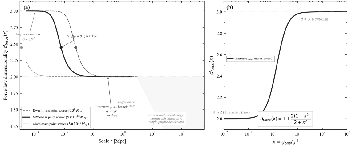
Synthetic benchmark inputs: g^\dagger = 1.2 \times 10^{-10} \text{ m s}^{-2} and idealized point-source masses; no observational data overlay; faded isolation cutoffs are display-only.
