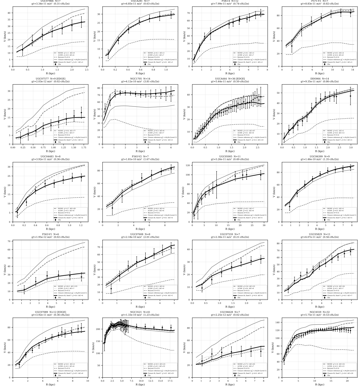
Figure 22: Representative SPARC rotation curves fitted with the new ECT galactic closure in the fixed- M/L mode. Black points with error bars show the observed rotation velocities. The baryons-only Newtonian contribution is shown separately, together with the best-fit ECT curve, the baseline ECT curve corresponding to g_0^\dagger = cH_0/(2\pi) , and the MOND and \Lambda CDM comparison curves produced by the same numerical pipeline. Where displayed, auxiliary fit statistics such as \chi^2_r and AIC are shown for visual comparison only. The fits use the new algebraic closure (17.24), not the older empirical RAR interpolation used in preliminary versions of the manuscript.
