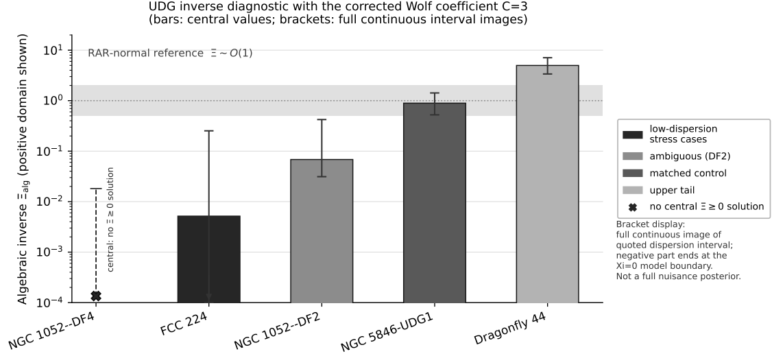
Figure 28: Corrected inverse-problem diagnostic for the adopted Level-C galactic closure at five spherical reference objects. The plotted quantity is the algebraic \Xi_{alg} required by the central Wolf proxy and the quoted dispersion interval at fixed (M_*, R_e) . A boundary marker is used where the algebraic result is negative: DF4 has no admissible \Xi \geq 0 solution at its central inputs. FCC 224 requires a small positive value, NGC 5846-UDG1 is near unity, and Dragonfly 44 is above unity. These are diagnostic proxy outputs, not an ECT prediction or a joint nuisance posterior; AGC 114905 requires a disc solver.
