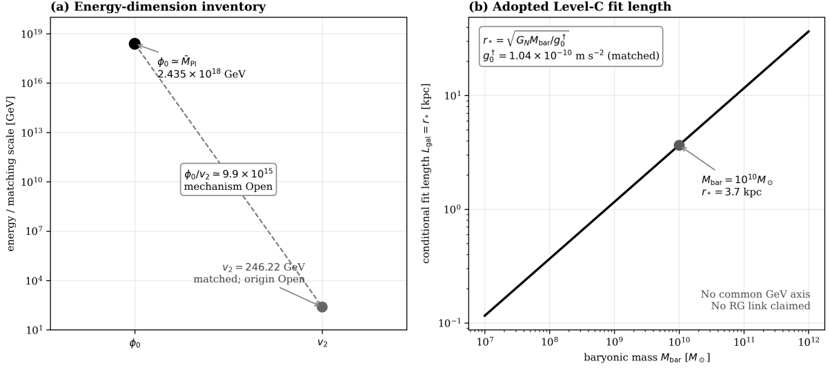
Figure 3: Dimensionally separated scale inventory. Left: the energy/matching quantities \phi_0 \sim \bar{M}_{Pl} and v_2 \sim 246 GeV; their ratio is displayed without claiming an RG derivation. Right: the conditional Level-C fit length L_{gal} \equiv r_* = \sqrt{G_N M_{bar} / g_0^\dagger} versus baryonic mass for the matched benchmark g_0^\dagger = cH_0 / (2\pi) . The right panel is closure algebra, not a third VEV, energy scale, or scalar-action prediction.
