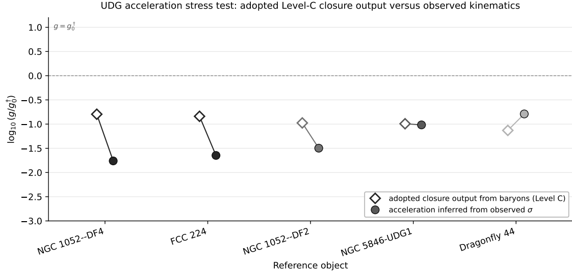
Figure 27: Direct object-by-object stress test of the adopted Level-C galactic closure. Open diamonds show the acceleration g_G computed from the baryonic g_N at the baseline g_0^\dagger ; filled circles show g_{\text{obs}} inferred from the measured velocity dispersion at R_{1/2} . The vertical coordinate is \log_{10}(g/g_0^\dagger) and the horizontal coordinate is the object identity, not a scalar-field coordinate. Connector segments expose the closure residual; corrected numerical inputs and the dispersion-only boundary audit are given in Appendix AT.
