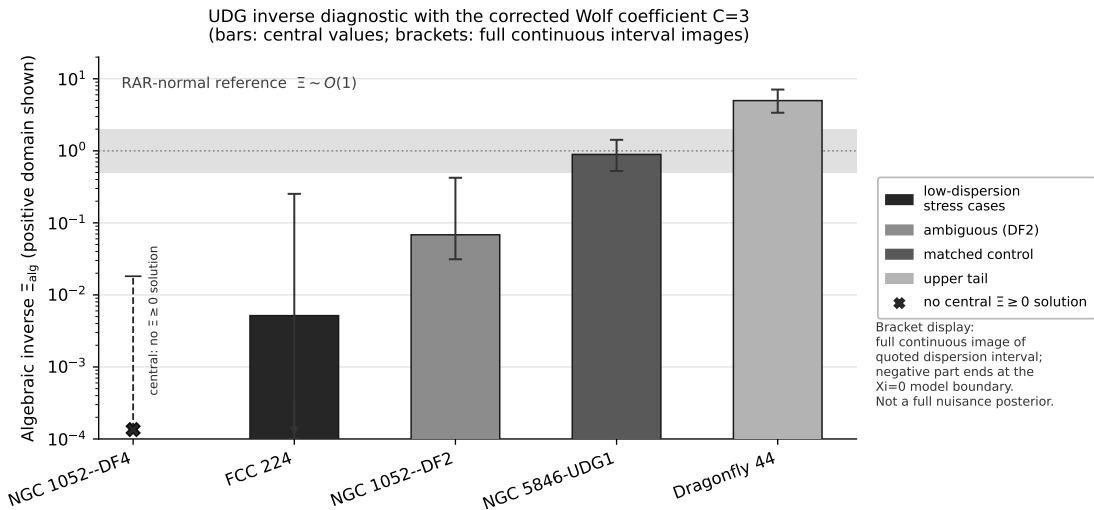
Figure 12: Corrected \Xi_{\text{alg}} inverse diagnostic. The DF4 boundary marker denotes no physical nonnegative- \Xi solution at the central inputs. Quoted-dispersion ranges are boundary checks, not a common 95% nuisance posterior. All results are Level C proxy algebra; the environment law is Open.
