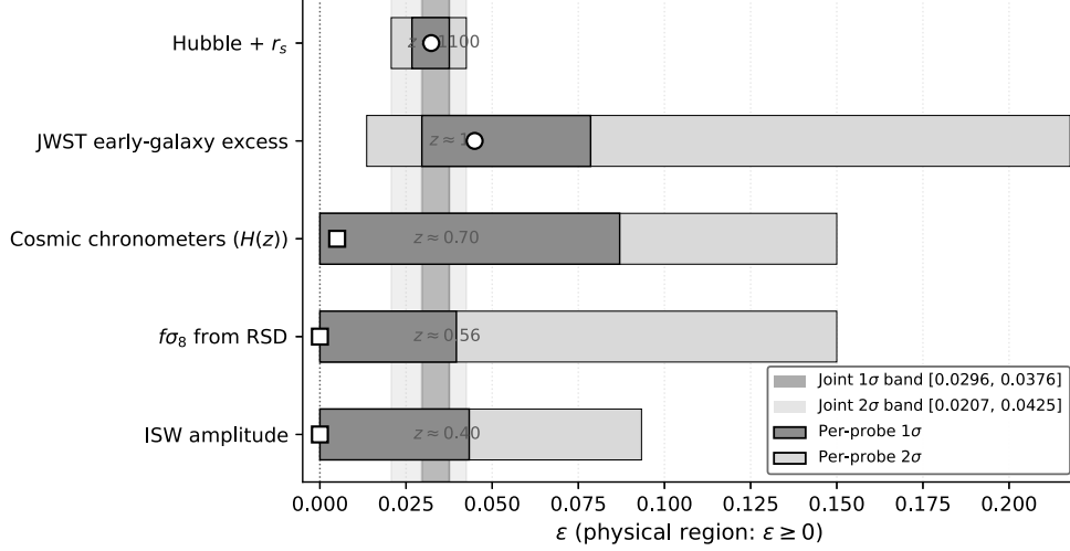
Figure 6: Summary of the five retained ECT diagnostic-layer channels that constrain the effective drift parameter \varepsilon : Hubble + r_s (acoustic scale + local ladder), JWST early-galaxy excess (growth + time-budget), cosmic chronometers (passive-galaxy ages), f\sigma_8 (redshift-space distortions), and the Integrated Sachs–Wolfe cross-correlation. Each channel yields a retained effective interval inside the shared diagnostic module; the intervals are not statistically independent likelihoods. The hatched band shows the common region, \varepsilon \in [0.0296, 0.0376] at 1\sigma . The lower edge is set by JWST and the upper edge by Hubble + r_s . ( Level B for the diagnostic-layer synthesis; not a first-principles ECT prediction. )
