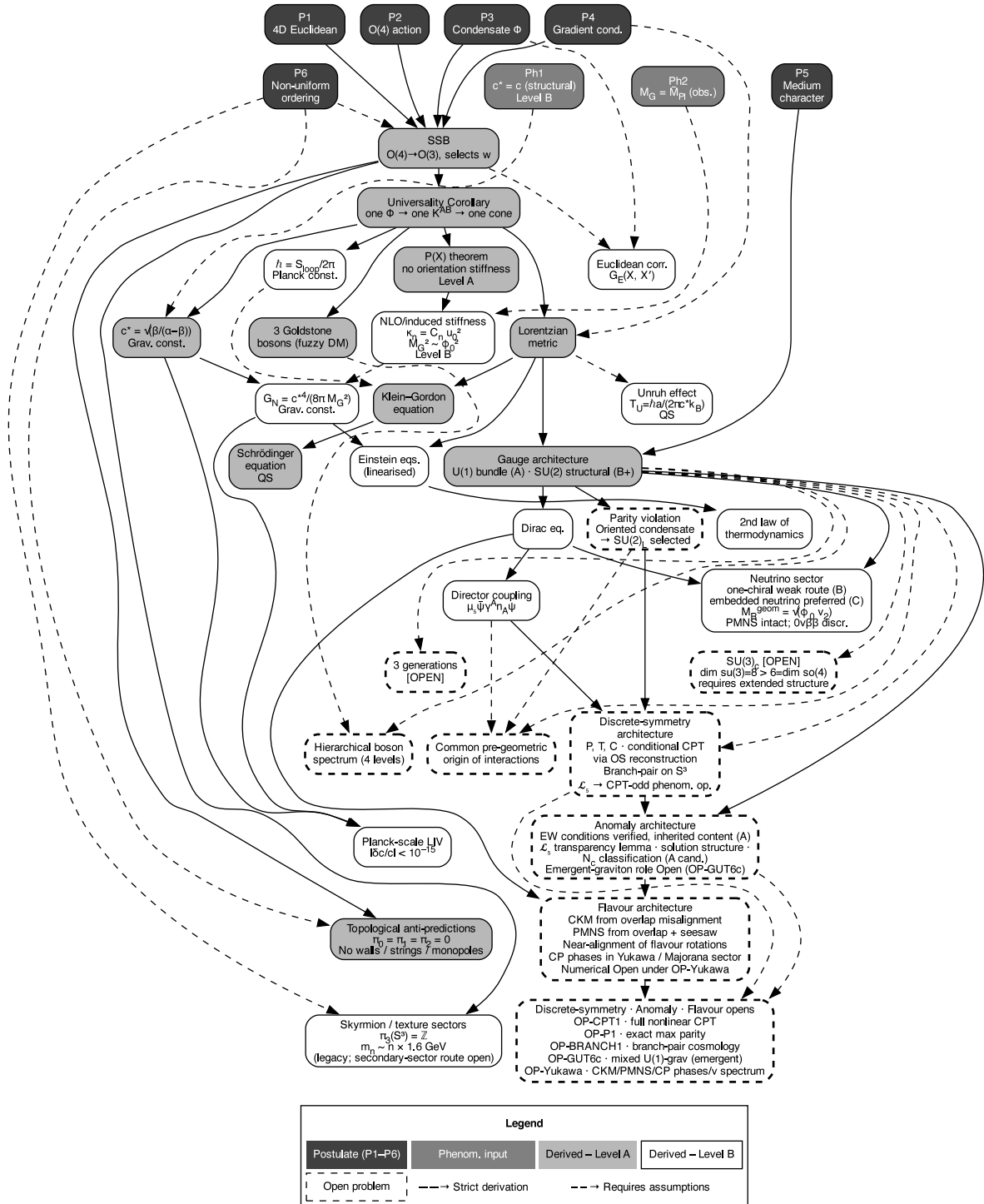
Figure 4: Part I derivation logic. From six postulates and BR1, the theory derives or structurally motivates: Lorentzian signature, universal causal cone, equation hierarchy, the retarded arrow-of-time backbone, the Level B entropy-growth closure, branching into geometric and coherent sectors, gauge-sector routes, particle-sector reconstruction targets, and compact-phase quantisation. Colours indicate Level A, B, and Open status.
