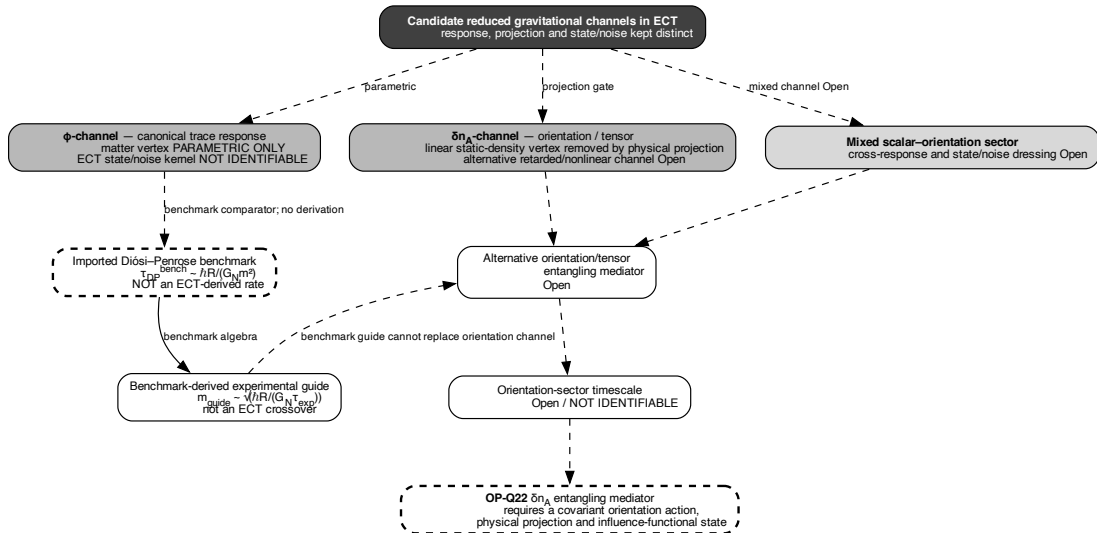
Figure 17: Operational taxonomy for candidate gravity-related record channels. The scalar trace vertex is parametric, while its state/noise kernel and finite-body charge are Open. The orientation/tensor route lacks a derived density projector and a specified state. The displayed Diósi–Penrose timescale \tau_{\text{dec}}^{\text{grav}} \sim \hbar R / (G_N m^2) and m_{\text{guide}} \sim \sqrt{\hbar R / (G_N \tau_{\text{exp}})} are imported benchmarks, not ECT-derived rates or crossover predictions. (Level C/Open.)
