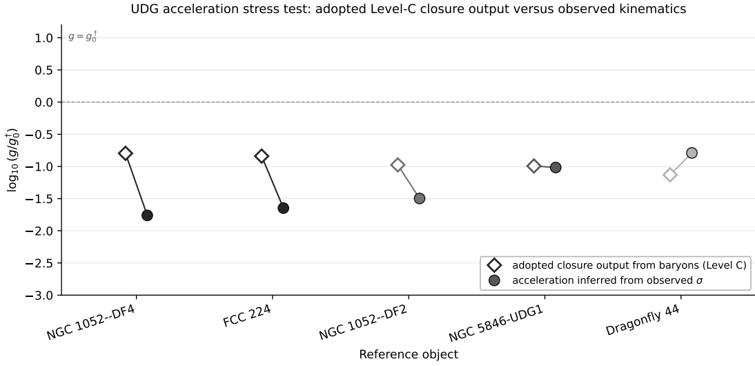
Figure 11: Direct acceleration-residual view for the UDG reference objects. The comparison uses g_{\text{obs}} = 3\sigma^2/R_{1/2} and the adopted Level-C closure; it assigns no microscopic scalar coordinate and is not a screening result.
