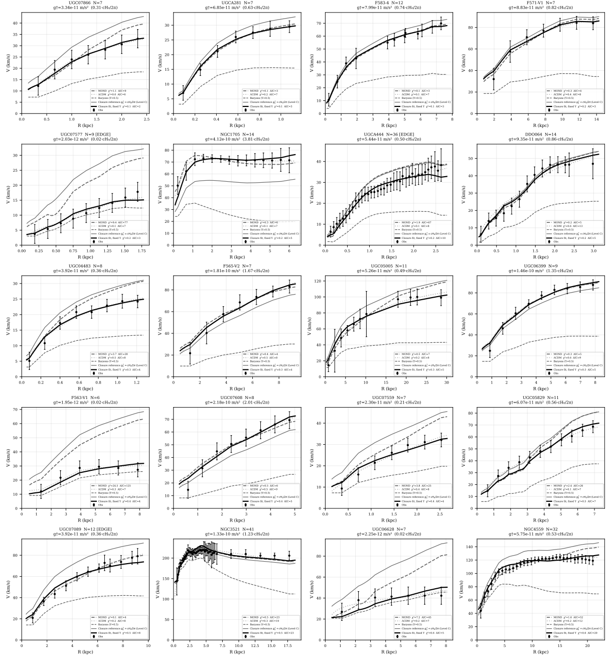
Figure 8: Rotation-curve fits for a sample of SPARC galaxies, spanning a wide range of morphologies: from dwarf irregulars to massive spirals. The adopted interpolation closure (solid) uses one fitted parameter per galaxy. ( Level C .)
