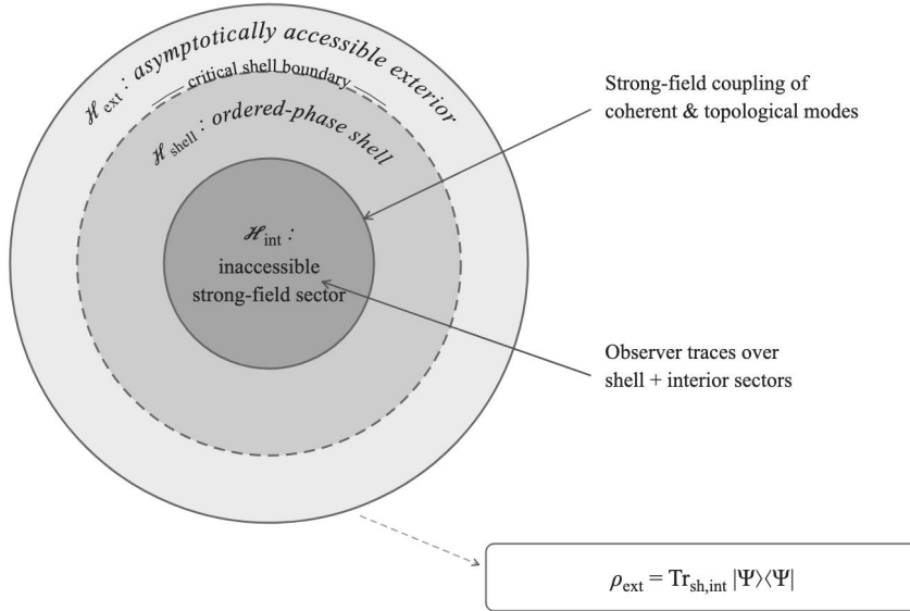
Figure 18: Candidate Level-B critical-shell picture. A shell/interface may replace the classical horizon inside this closure, while its geometry, correlations, and Euclidean-core continuation remain Open. No fundamental information destruction is an architecture-level postulate; a constructive outgoing-correlation recovery is not derived.
