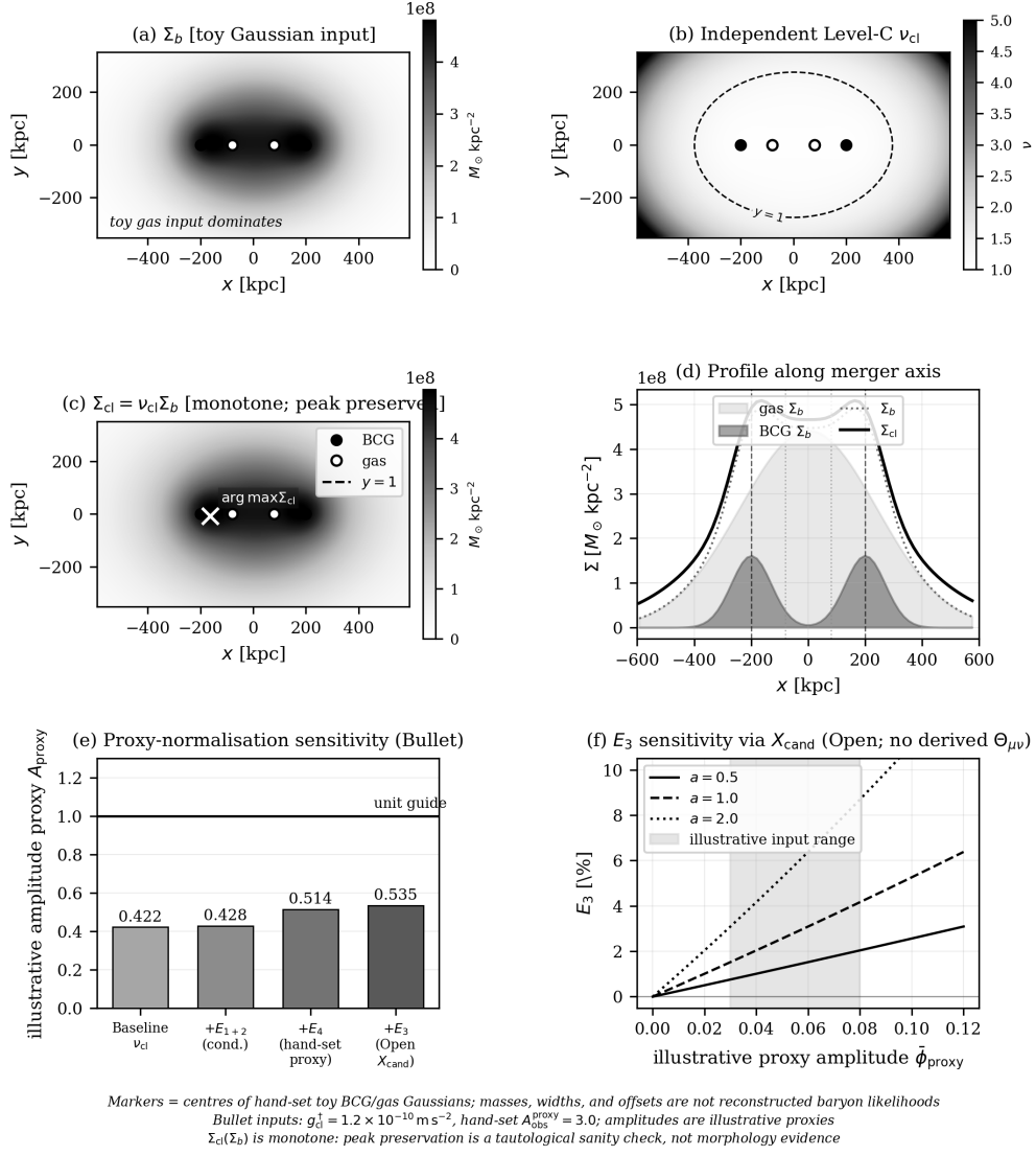
Figure 13: Bullet-cluster local-map audit. The proxy peak must coincide with the hand-set baryonic-map peak by exact monotonicity. Normalisation and orientation entries are hand-set/external sensitivities, not observed mass ratios.
