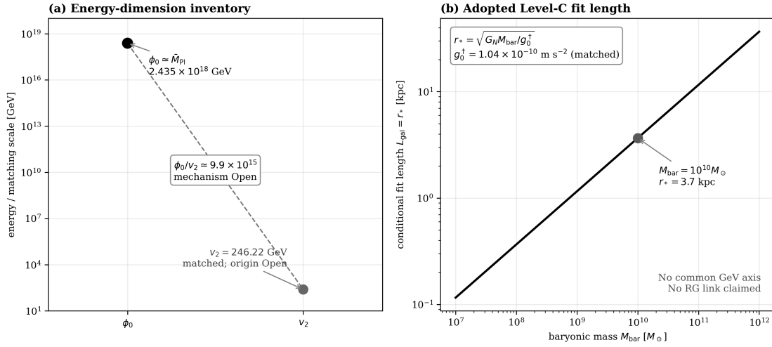
Figure 3: Dimensionally separated scale inventory. The left panel compares the two energy-dimension quantities \phi_0 and v_2 ; the gradient amplitude u_0 has units \text{GeV}^2 and is related only by the conditional dimensional estimate u_0 \sim \phi_0 m_\sigma . The right panel shows the distinct length L_{\text{gal}} = r_* = \sqrt{G_N M_{\text{bar}}/g^\dagger} inside the adopted Level-C galactic functional. No common-axis RG flow or first-principles bridge among these objects is claimed.
