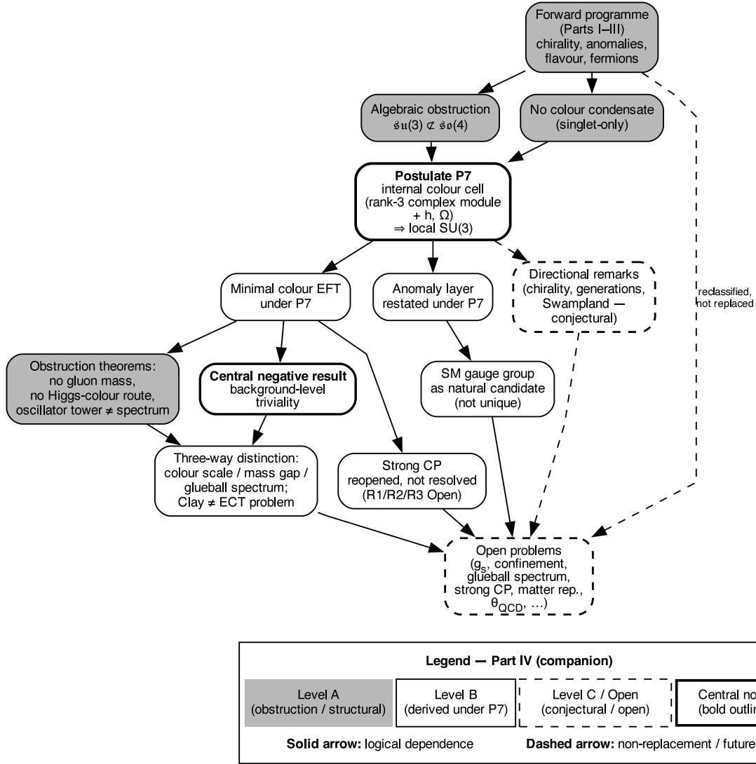
Figure 20: Part IV derivation logic at a glance. Starting from the forward programme of Parts I–III, two obstruction theorems force the externalisation of colour; the reverse-engineered postulate P7 equips the medium with an internal colour cell carrying exact local SU(3) . Two branches follow: a minimal admissible colour effective theory (with obstruction theorems and a central negative result — background-level triviality) and an anomaly layer yielding the Standard-Model gauge group as a natural candidate. The three-way distinction (colour scale vs mass gap vs glueball spectrum) is sharpened in the preprint into a separation of the physical mass-gap question, for which a conditional theorem is given, from the mathematical Clay problem, whose continuum object is shown not to be fundamental in ECT; the strong-CP problem is reopened rather than resolved. Apart from one explicitly marked Level A meta-statement (that the Clay continuum object is not a fundamental object of ECT), everything in Part IV is Level B or C.
