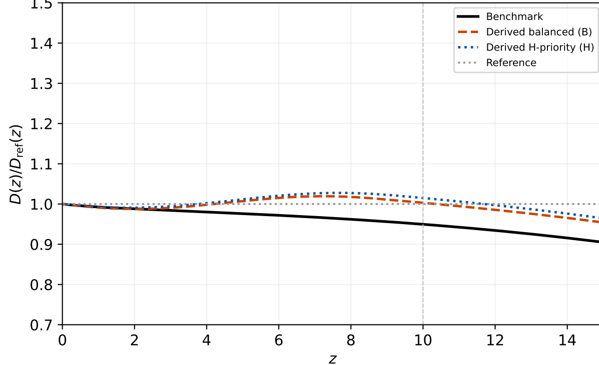
(c) Solved linear growth factor
