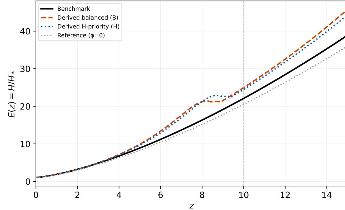
(a) Expansion history
