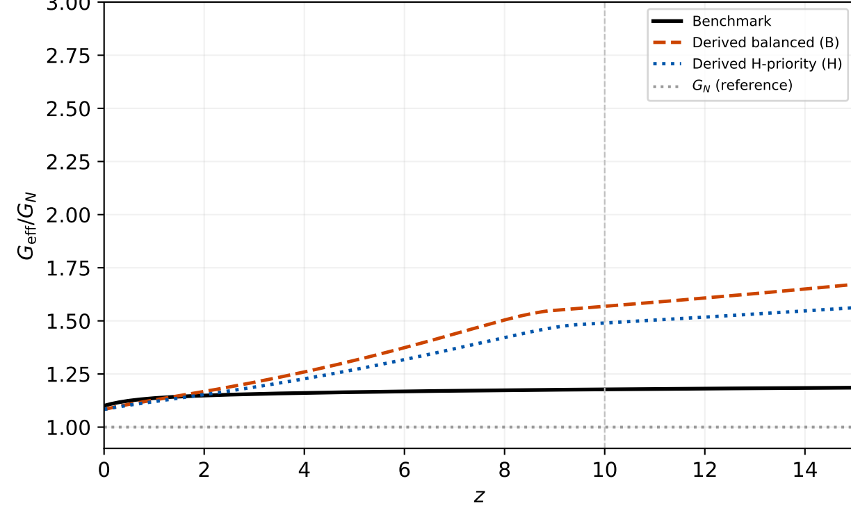
(b) Effective gravity
