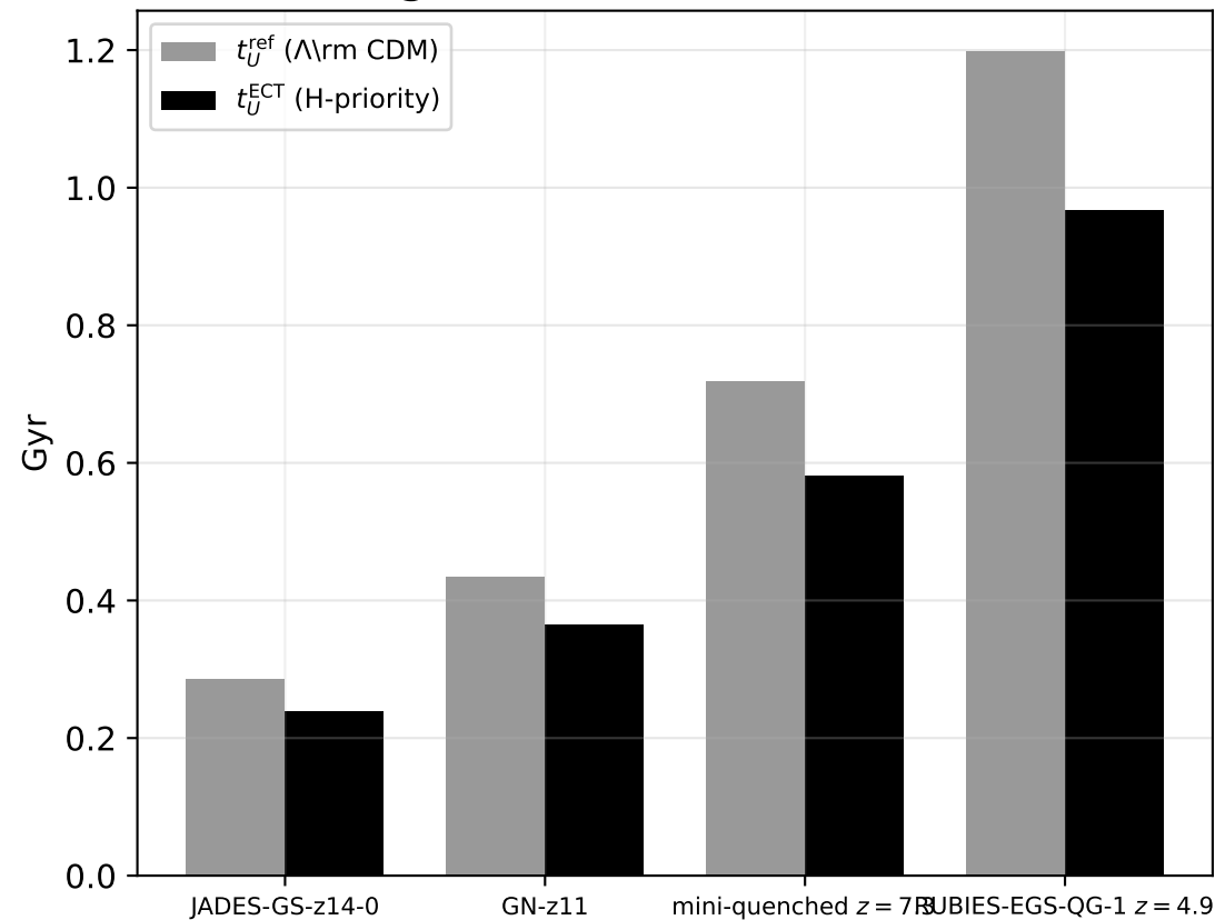
(a) Age of Universe at observation
