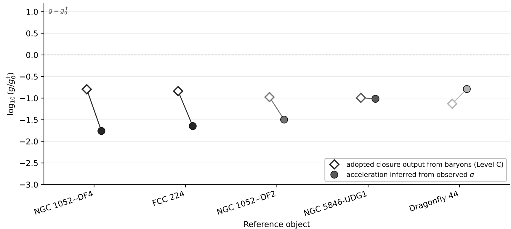
UDG acceleration stress test: adopted Level-C closure output versus observed kinematics
