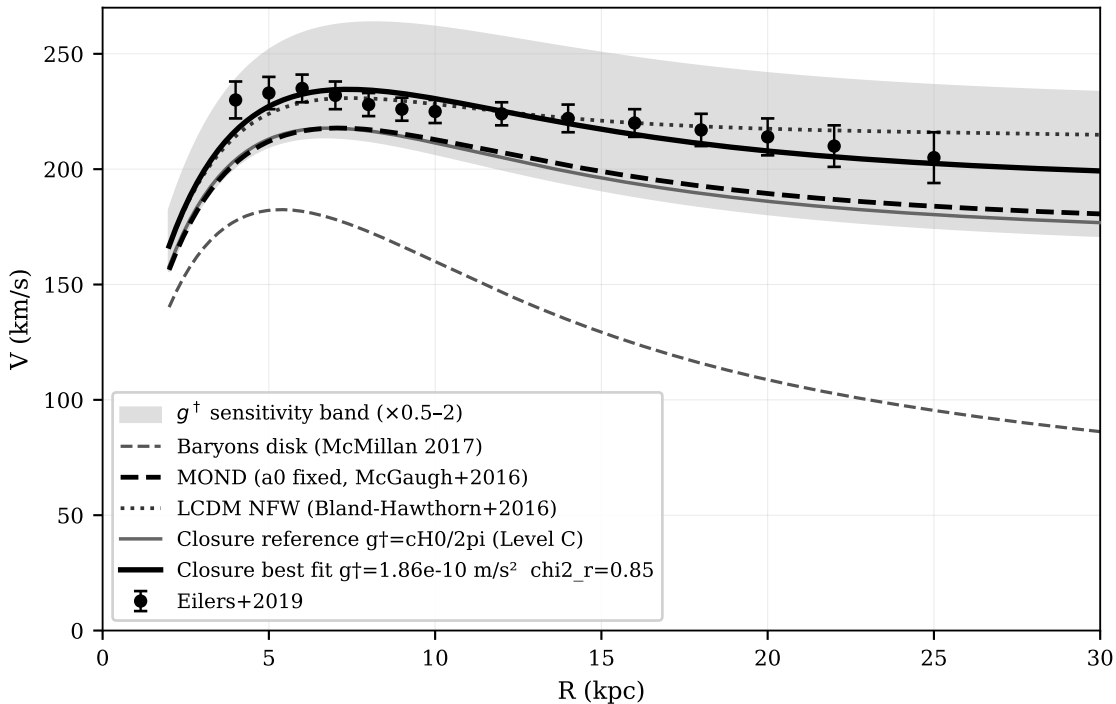
Milky Way rotation-curve fit — adopted Level-C galactic closure g^\dagger_{\text{fit}} = 1.86 \times 10^{-10} \text{ m/s}^2 = 1.72 \times cH_0/2\pi \chi^2_r = 0.85
