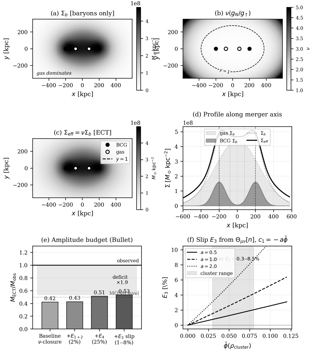
Filled circles = BCG (collisionless); open circles = X-ray gas (collisional)
