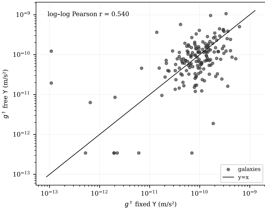
Fixed-ML vs free-ML g^+ (M/L degeneracy check)
