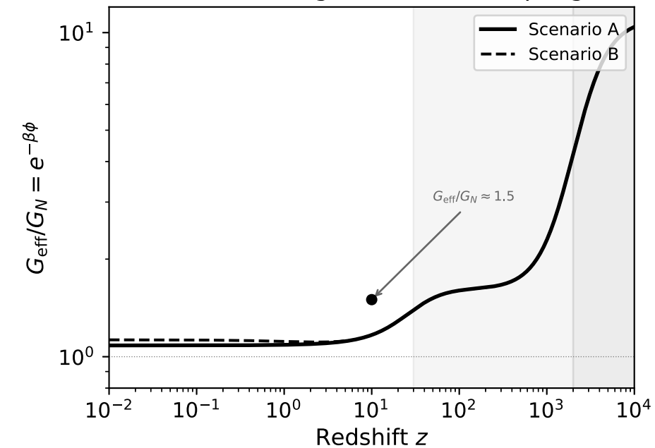
(c) Effective gravitational coupling
