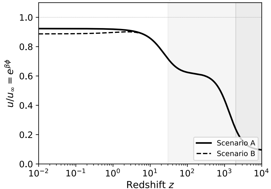
(b) Condensate amplitude ratio
