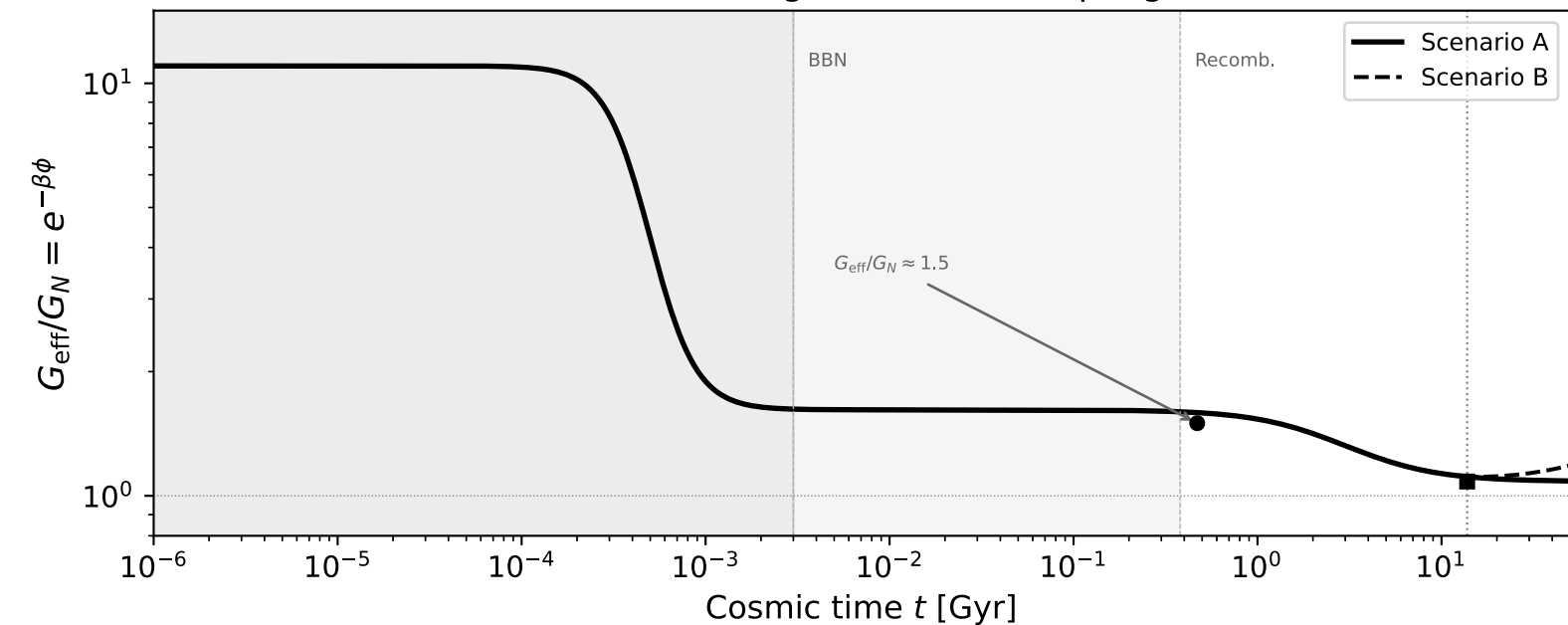
(b) Effective gravitational coupling
