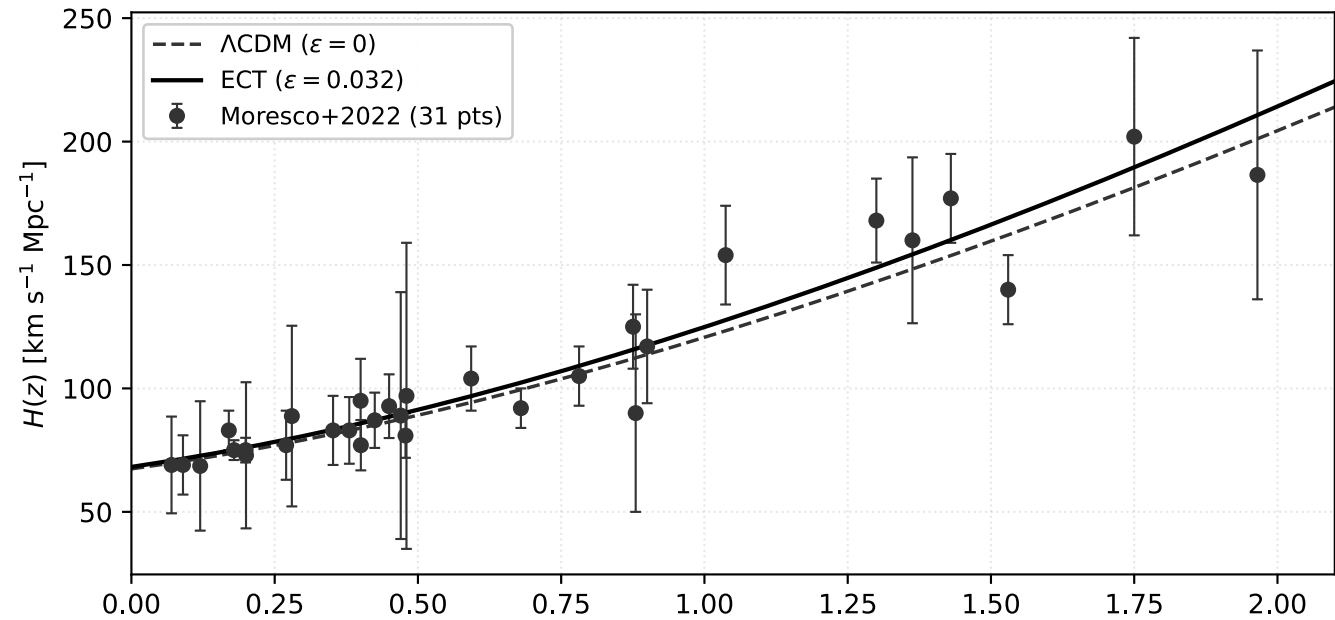
Cosmic chronometers H(z) : data vs. ECT model
