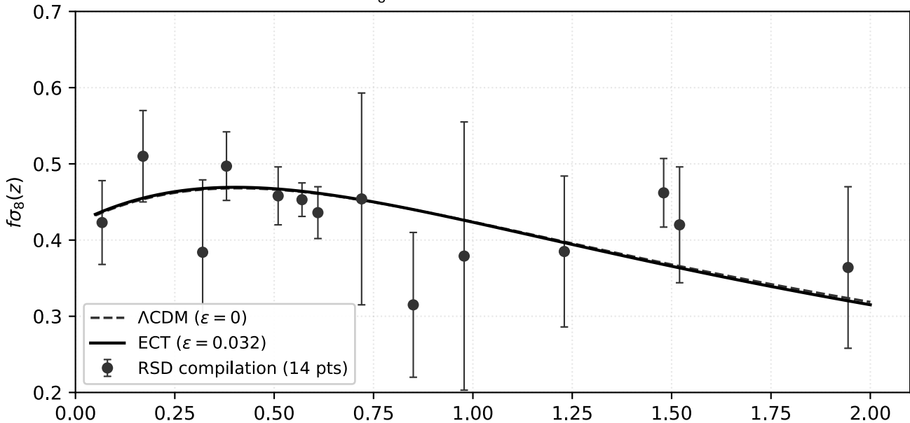
f\sigma_8 RSD: data vs. ECT model
