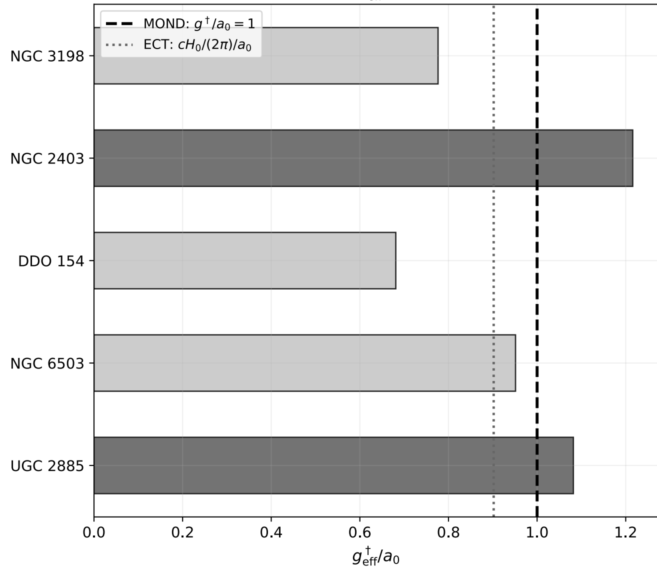
(b) Deviation of g_{\text{eff}}^{\dagger} from universal a_0
