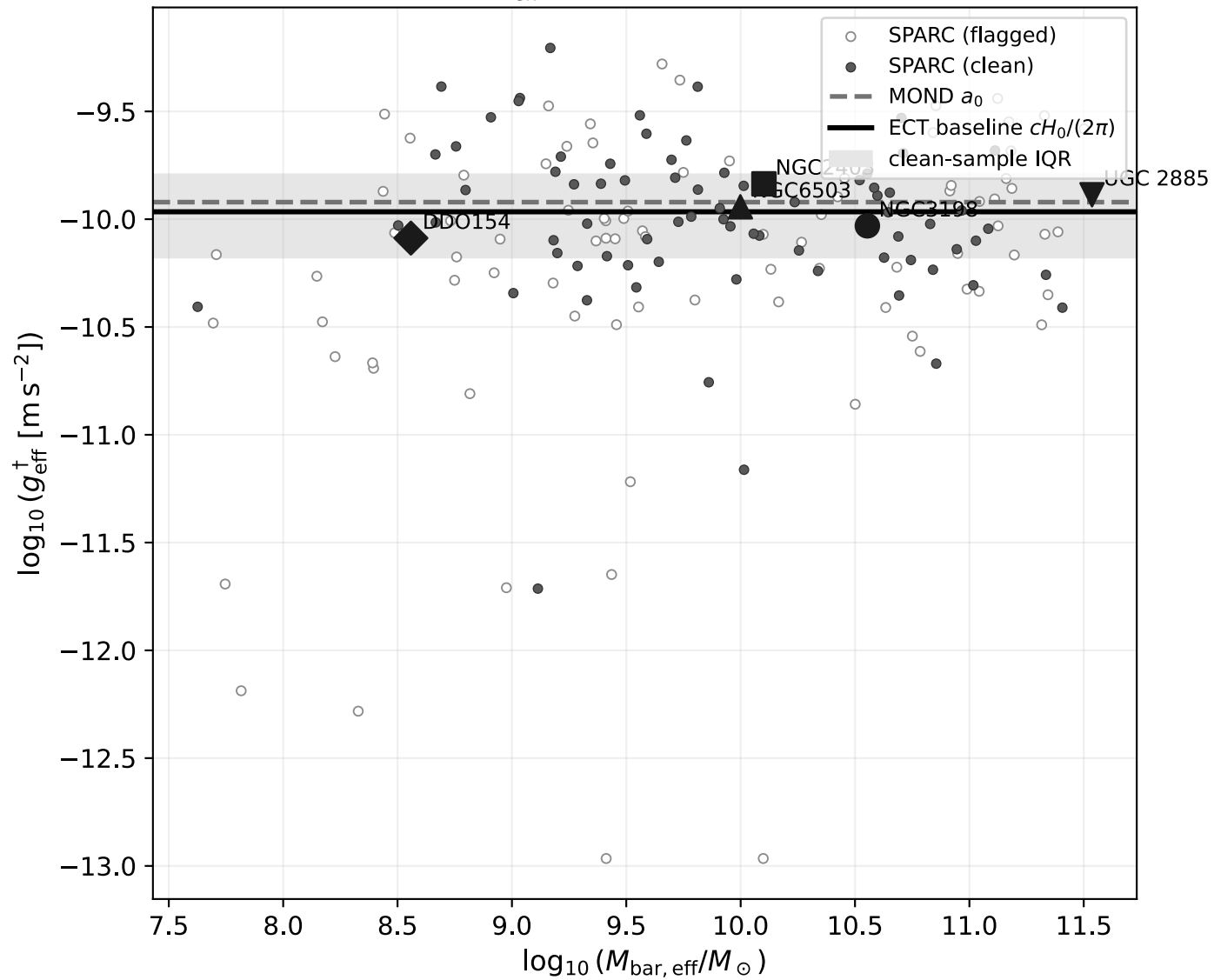
(a) Fitted g_{\text{eff}}^{\dagger} vs. effective baryonic mass
