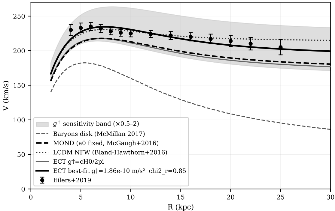
Milky Way rotation curve ECT phi-branch g^\dagger_{\text{fit}} = 1.86 \times 10^{-10} \text{ m/s}^2 = 1.72 \times cH_0/2\pi \chi^2_r = 0.85
