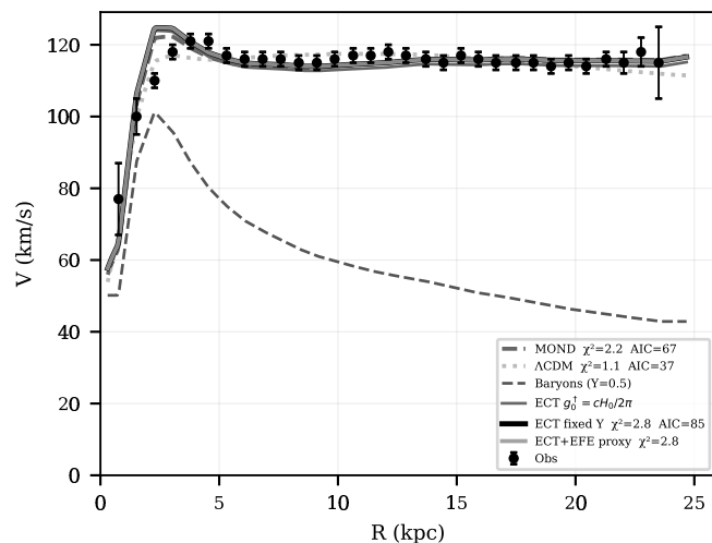
NGC6503 N=31 g\ddagger=1.14\text{e-}10 \text{ m/s}^2 \text{ (} 1.05\cdot cH_0/2\pi \text{)}
