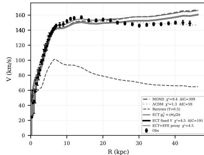
NGC3198 N=43 g\ddagger=9.32\text{e-}11 \text{ m/s}^2 \text{ (} 0.86\cdot cH_0/2\pi \text{)}
