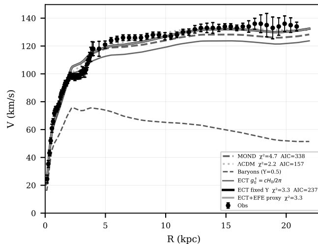
UGC02885 N=19 g\ddagger=1.30\text{e-}10 \text{ m/s}^2 \text{ (} 1.20\cdot cH_0/2\pi \text{)}
