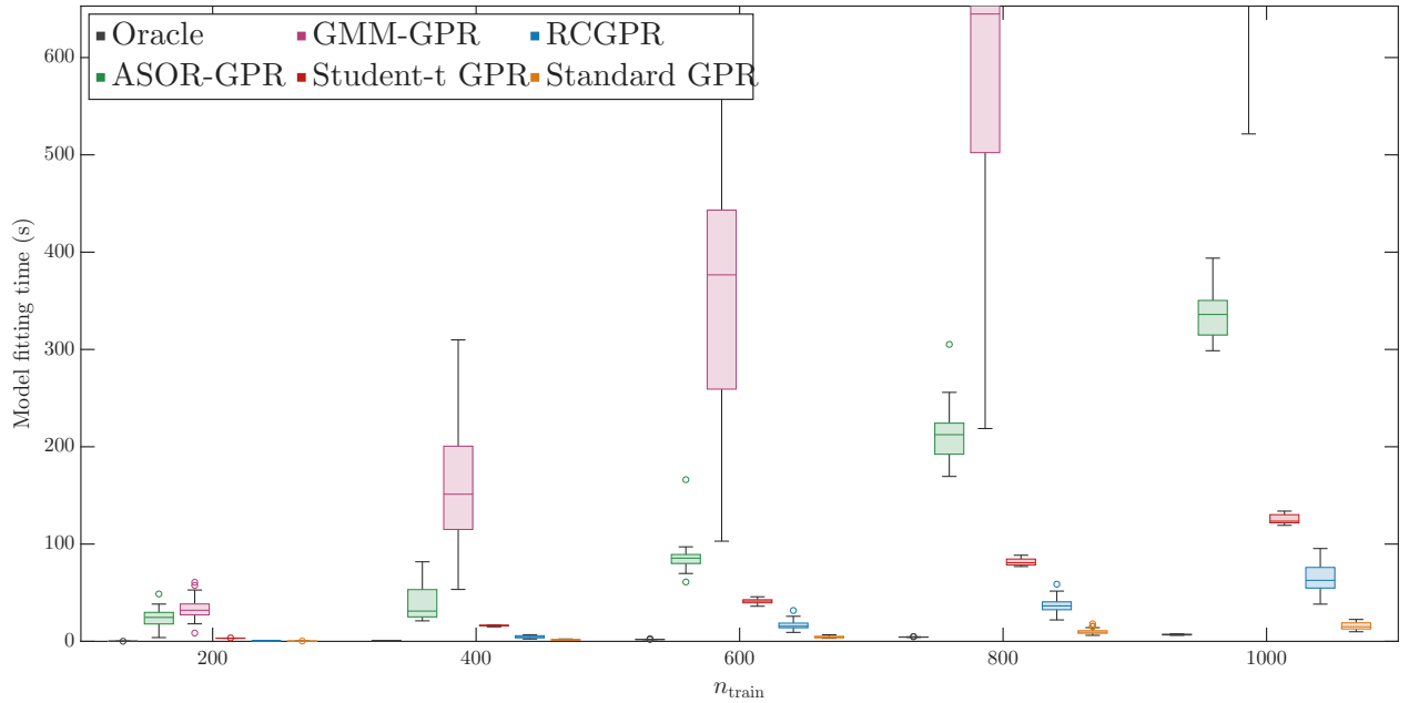
Figure 4. Serial model-fitting runtime as a function of the training-set size for the Oracle, ASOR-GPR, GMM-GPR, Student- t GPR, RCGPR, and standard GPR.
