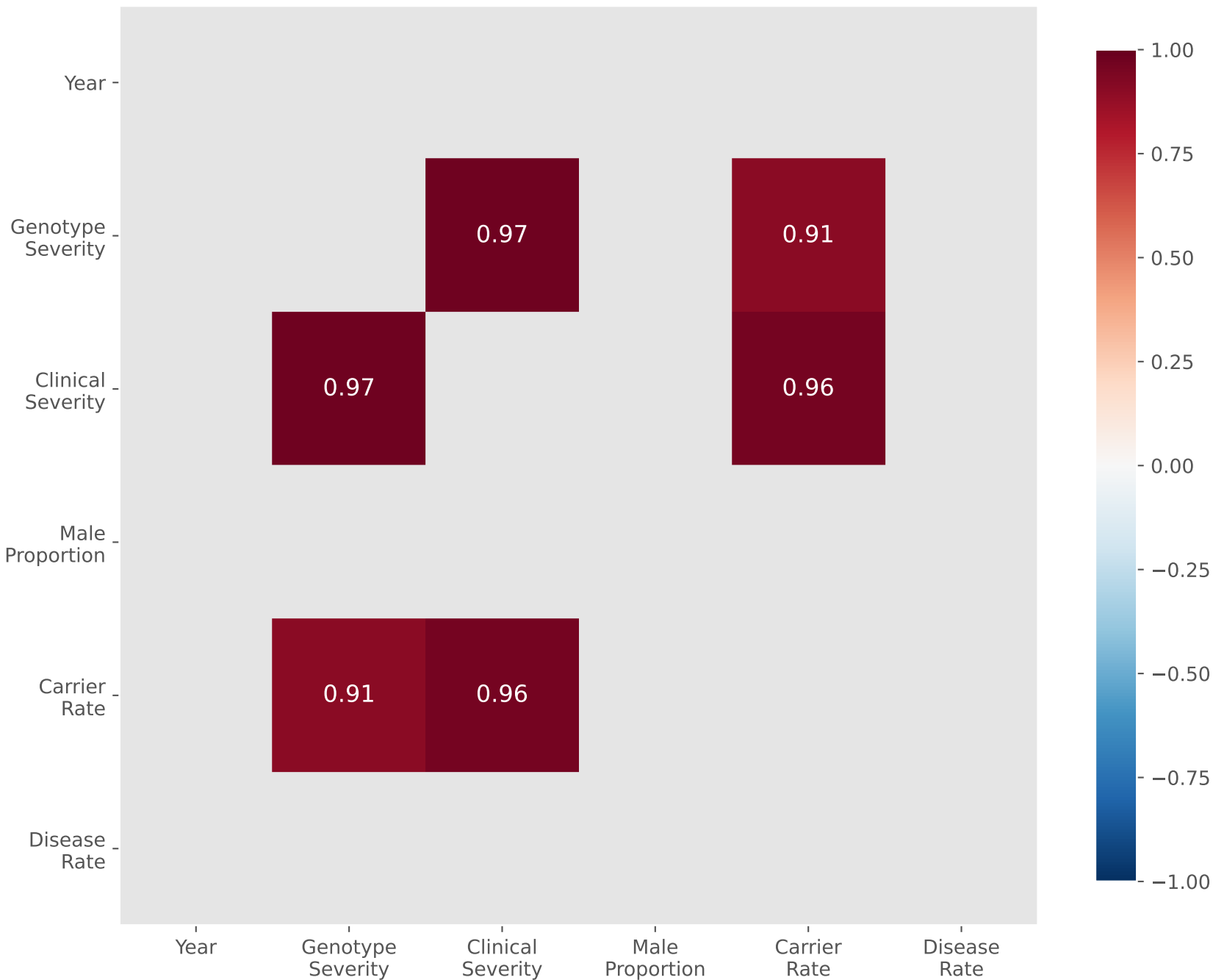
Fig. 4. Correlation Matrix with Non-significant Values Filtered ( p > 0.05 )
