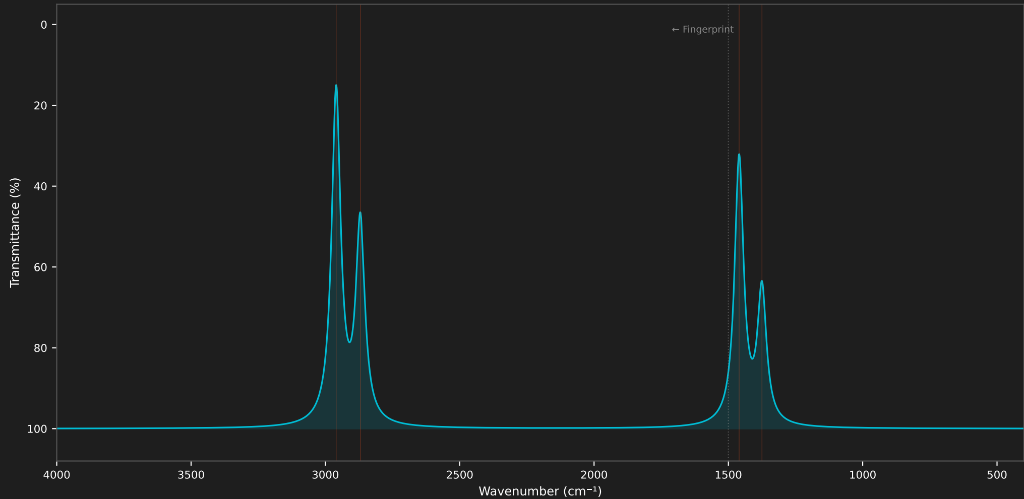
Predicted IR Spectrum (SMILES CC(=O)OCC )
