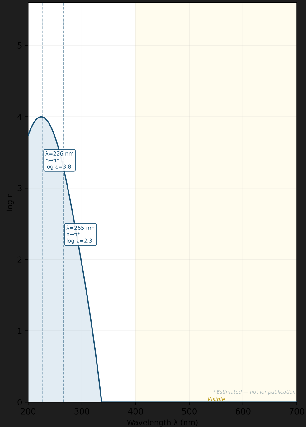
UV-Vis: \log \epsilon
