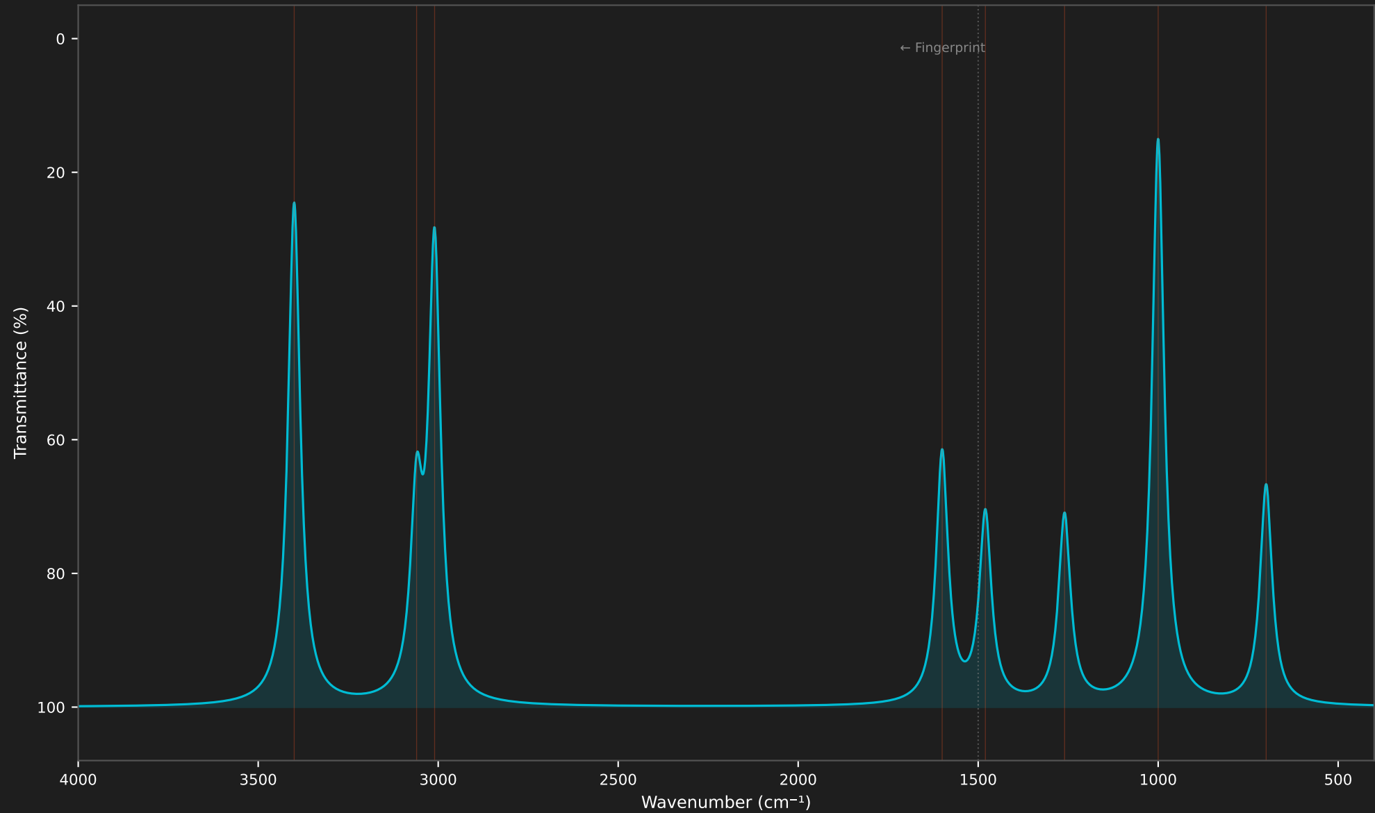
Predicted IR Spectrum (SMILES CC(=O)OCC )
