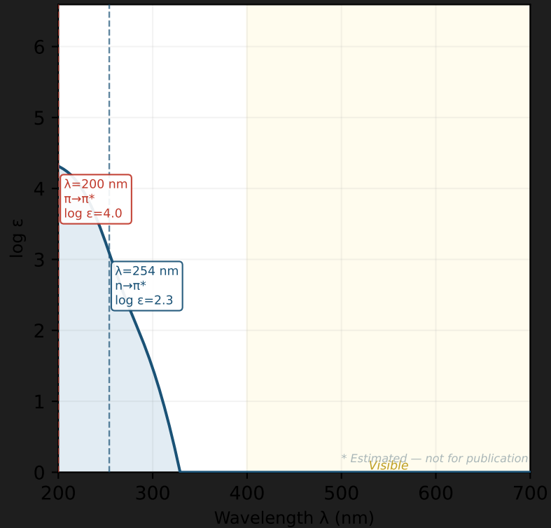
UV-Vis: \log \epsilon
