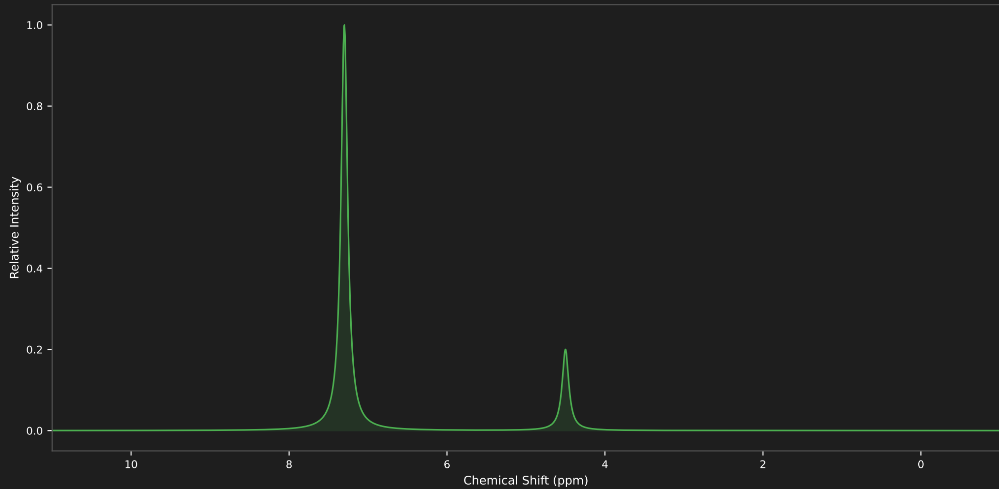
Predicted ^1\text{H} NMR Spectrum (SMILES CC1=CC=CC=C1 )
