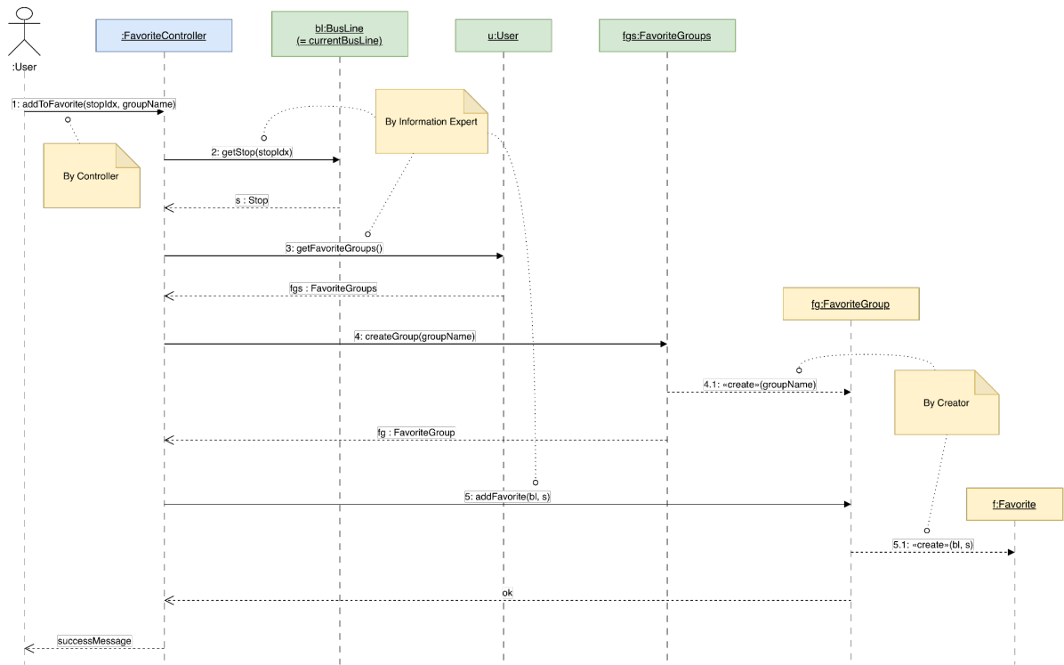
SD - addToFavorite(stopIdx, groupName)
