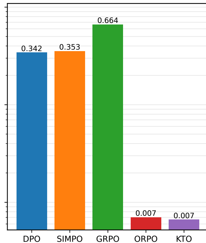
Qwen3-4B-Instruct-2507
