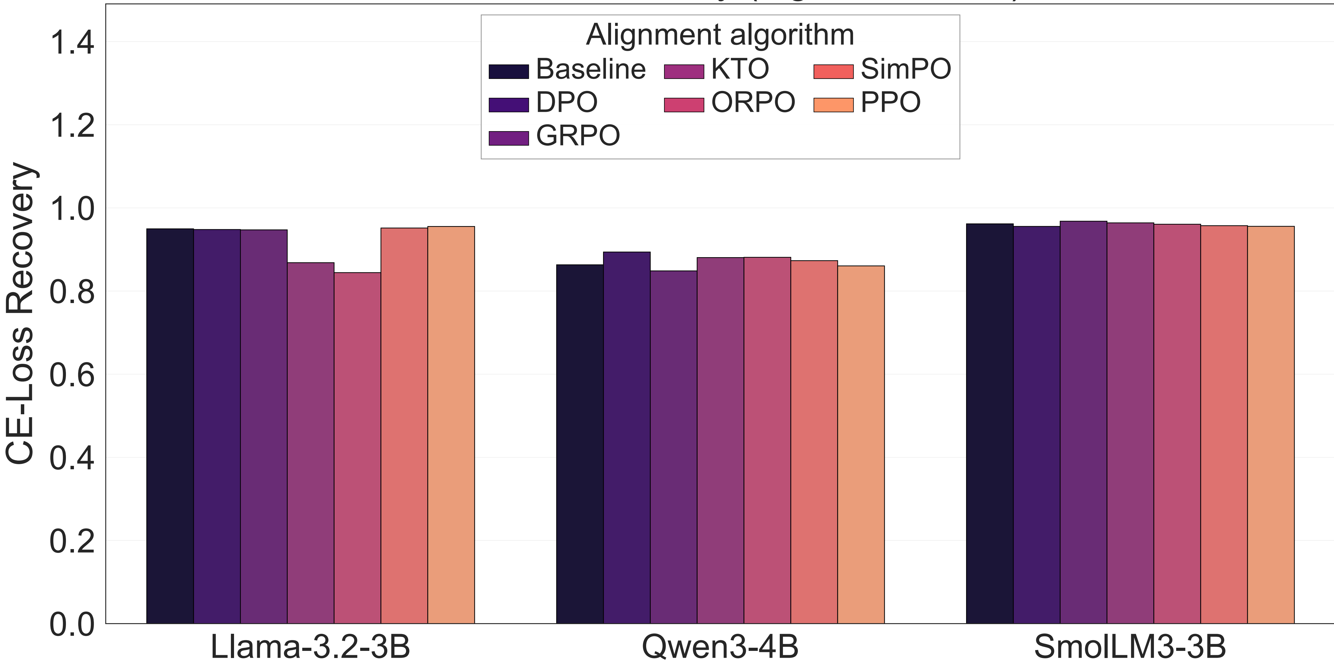
CE-Loss Recovery (higher is better)
