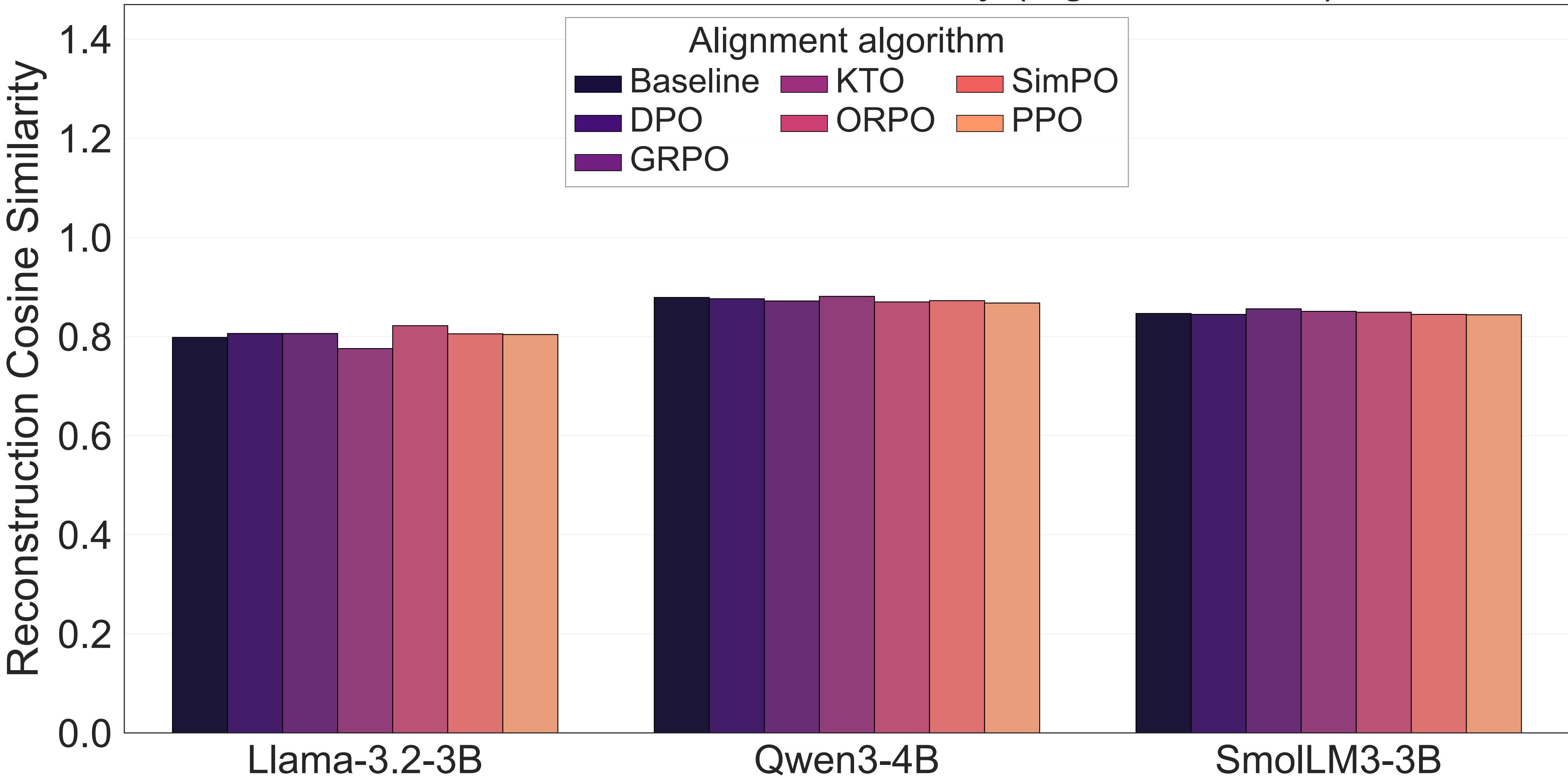
Reconstruction Cosine Similarity (higher is better)
