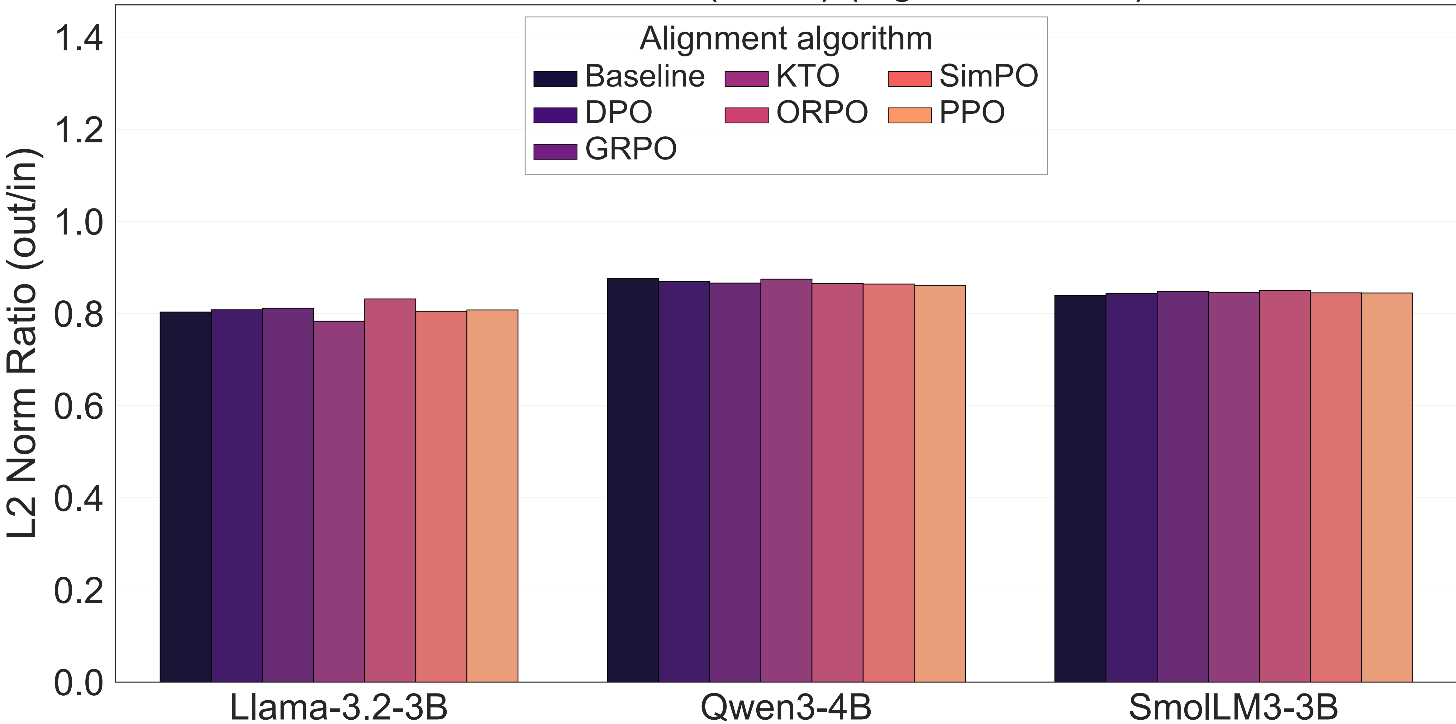
L2 Norm Ratio (out/in) (higher is better)
