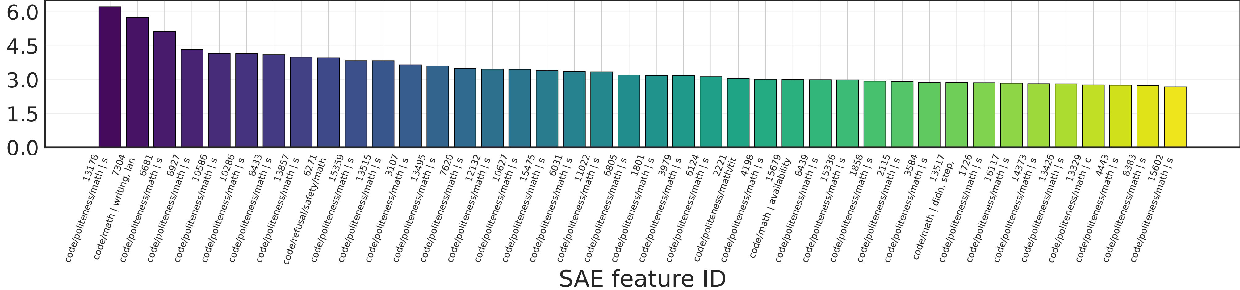
Top 40 features by mean activation (appendix) Qwen3-4B-ORPO (layer 22)
