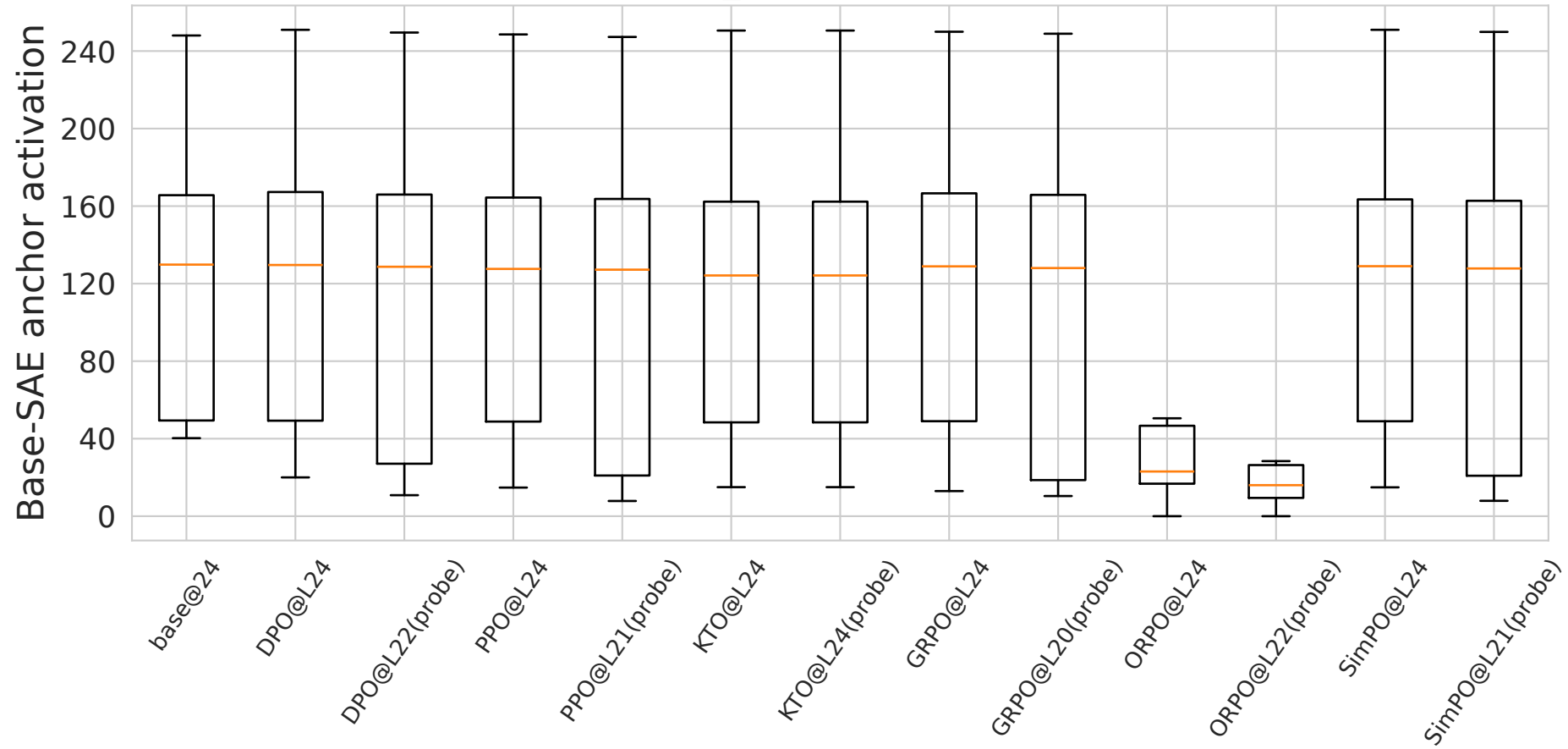
Anchor feature 6910 (Qwen3-4B-Instruct-2507) Readout: base_sae.encode(residual)[..., f]
