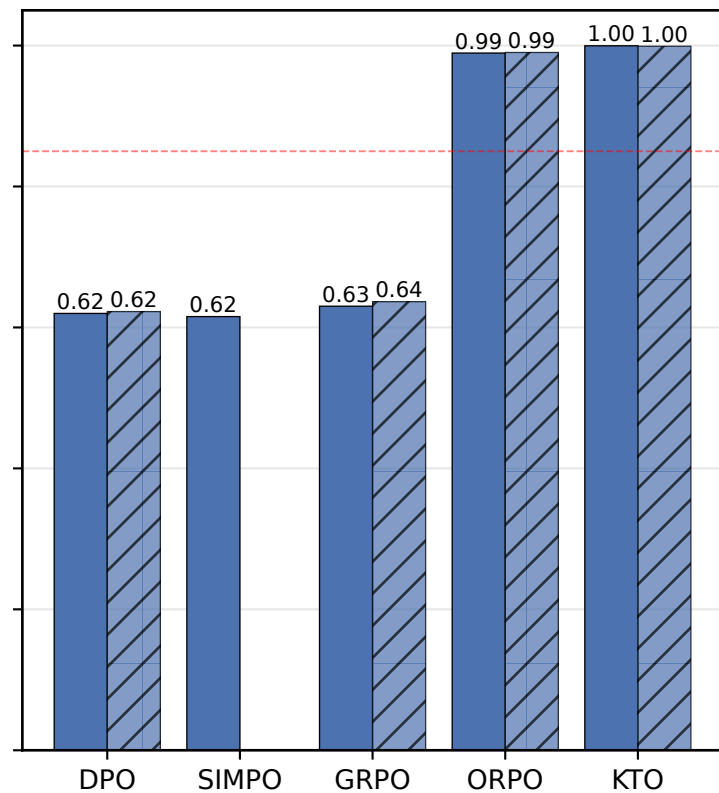
Qwen3-4B-Instruct-2507
