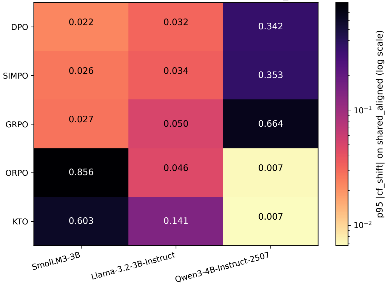
Per-feature shift magnitude (95th percentile) on shared_aligned class
