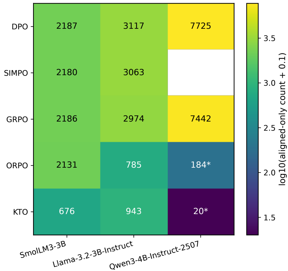
Aligned-only feature counts per (algorithm, base) heatmap. * = degenerate crosscoder.
