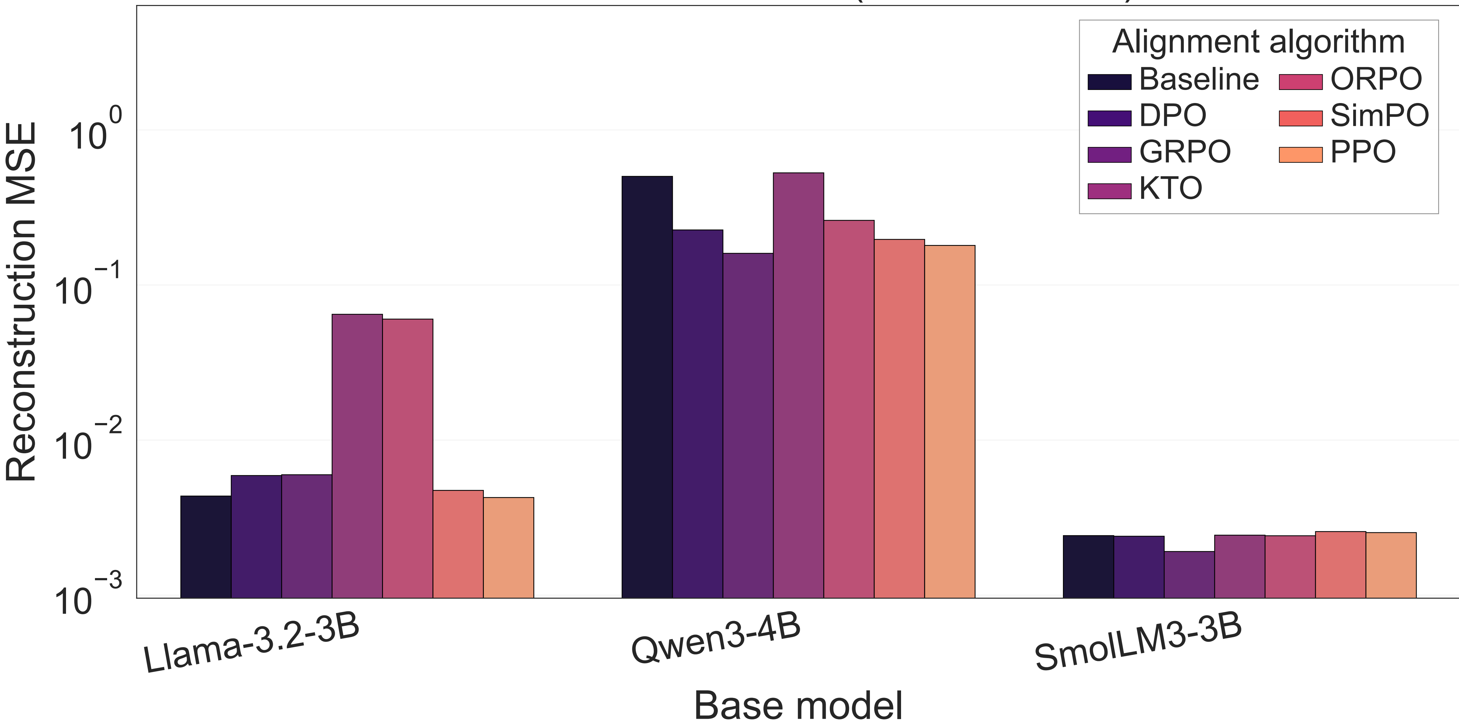
Reconstruction MSE (lower is better)
