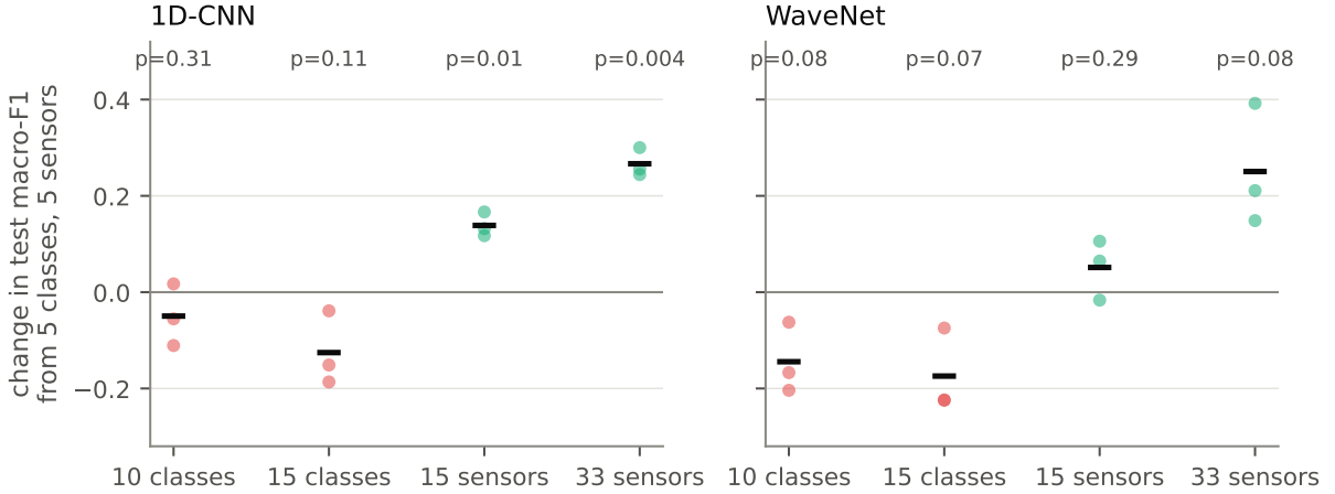
Figure 6: Change in test macro-F1 when the number of classes or of sensors is increased from a baseline of five classes and five sensors (Z24, single-channel input). Dots are individual splits; bars are means. More classes lower the score, more sensors raise it.
