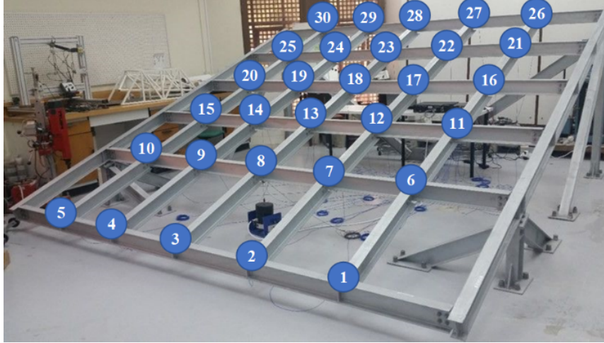
Figure 3: The QUGS steel frame with its thirty joints numbered. Each joint carries one accelerometer, and each damage state loosens the bolts at one joint. Source: QUGS benchmark, Qatar University.
