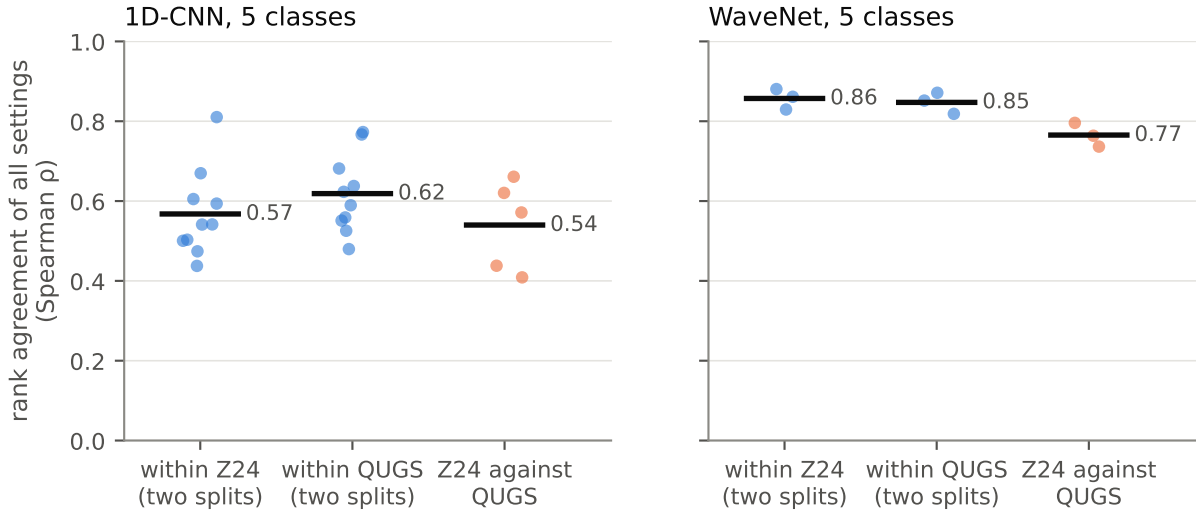
Figure 8: Rank agreement of all settings with five classes: between two splits of the same benchmark (blue) and between Z24 and QUGS (orange). Each dot is one pair of splits; bars are means.
