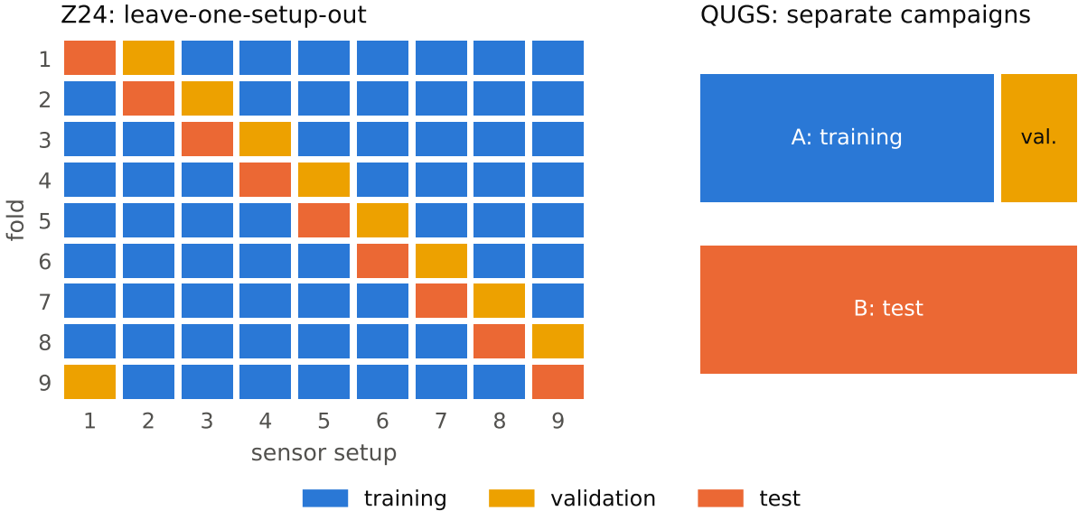
Figure 4: How the data are split. On Z24 each fold holds out one whole sensor setup for testing and the next one for validation; on QUGS training and validation use campaign A and testing uses all of campaign B.
