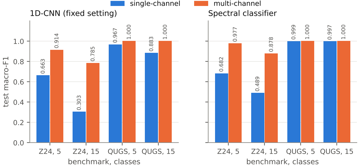
Figure 5: Test macro-F1 with single-channel and multi-channel input, for the 1D-CNN (left) and the spectral classifier (right). Both improve on Z24, which shows that the multi-channel input adds information rather than model capacity.
