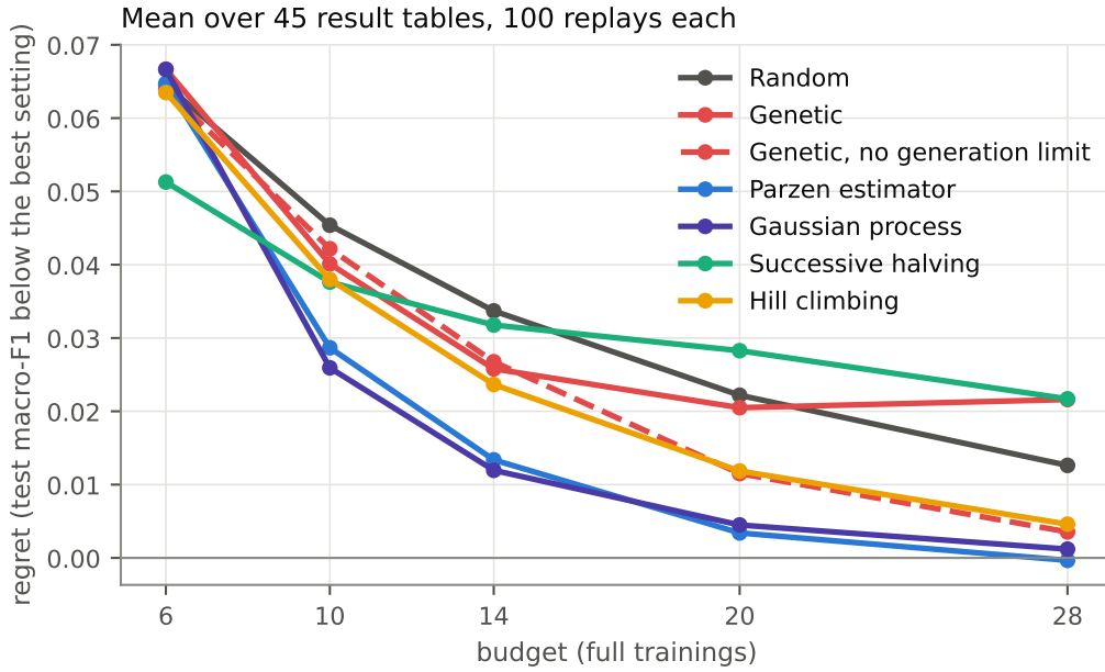
Figure 9: Regret of the seven search algorithms against the budget. Successive halving is best at six trainings, the two Bayesian methods from ten trainings onward, and the genetic algorithm with a fixed number of generations stops improving after about sixteen trainings.
