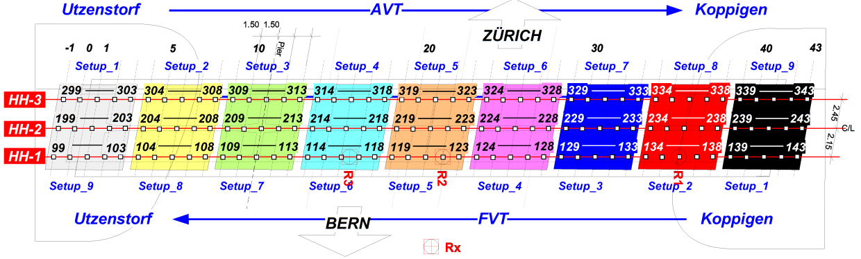
Figure 2: Sensor layout on the Z24 bridge deck, in plan view. Each coloured area is one of the nine sensor setups, with the numbered measurement points along three lines (HH-1 to HH-3). R1–R3 are the reference positions, where sensors stayed in place in every setup. AVT and FVT denote the ambient and forced vibration tests. Source: Z24 benchmark documentation, KU Leuven.
