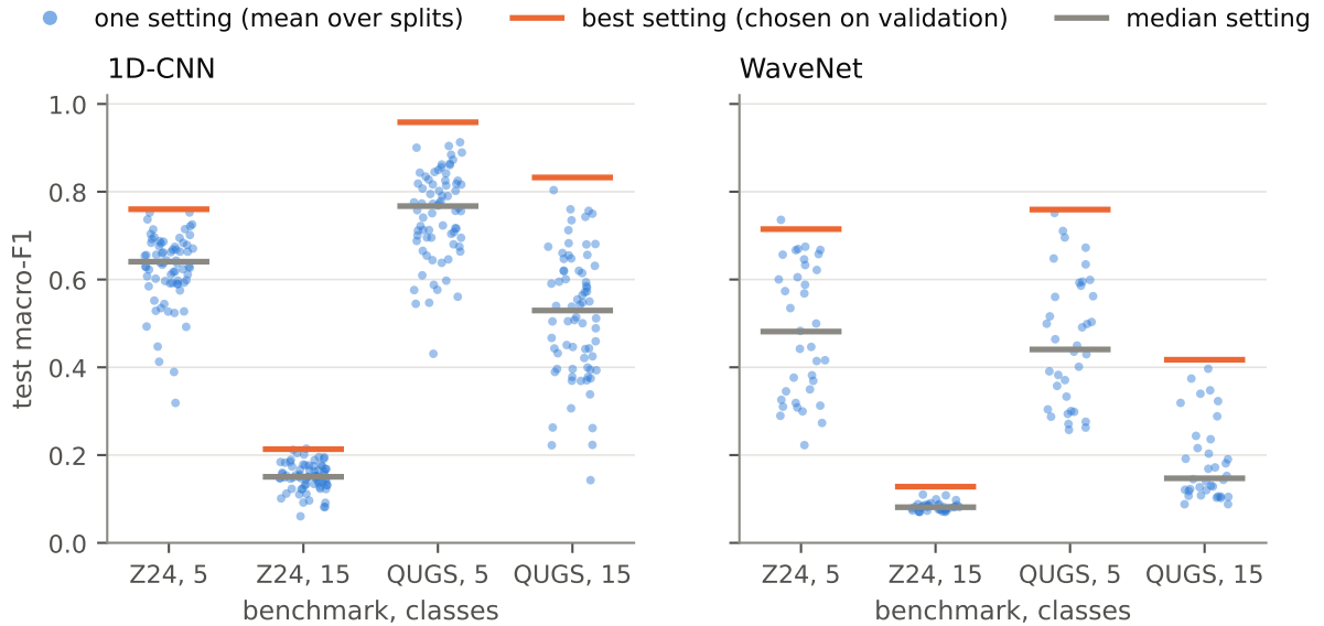
Figure 7: Test macro-F1 of every hyperparameter setting (dots, mean over splits), with the best setting chosen on validation data (orange) and the median setting (grey). The gap between the two lines is the value of tuning.
