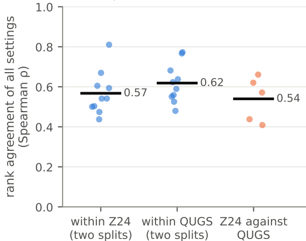
1D-CNN, 5 classes
