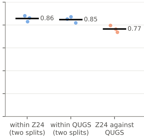
WaveNet, 5 classes
