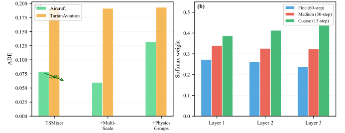
Fig. 4. (a) Component ablation with consistent model capacity. Multi-scale temporal mixing provides a 24.4% ADE reduction on Aircraft; on TartanAviation, all three configurations perform similarly, confirming that multi-scale acts primarily as a regularizer on small datasets. (b) Learned branch weights after softmax normalization. The coarse branch consistently receives the highest weight, increasing from 38.7% in Layer 1 to 43.7% in Layer 3.
