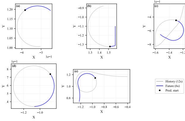
Fig. 3. Representative trajectory predictions on the Aircraft dataset. (a)–(e) Five test examples with increasing displacement magnitude. Gray: 12s history. Blue: 6s ground-truth future. Black dot: prediction start.
