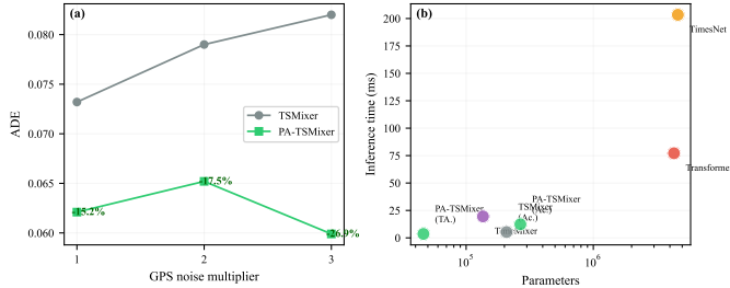
Fig. 5. (a) Noise robustness: PA-TSMixer’s relative advantage grows from -15.2\% to -26.9\% as GPS noise triples, due to implicit low-pass filtering in the pooled branches. (b) Computational efficiency: PA-TSMixer occupies the favorable lower-left region with low parameter count and fast inference.
